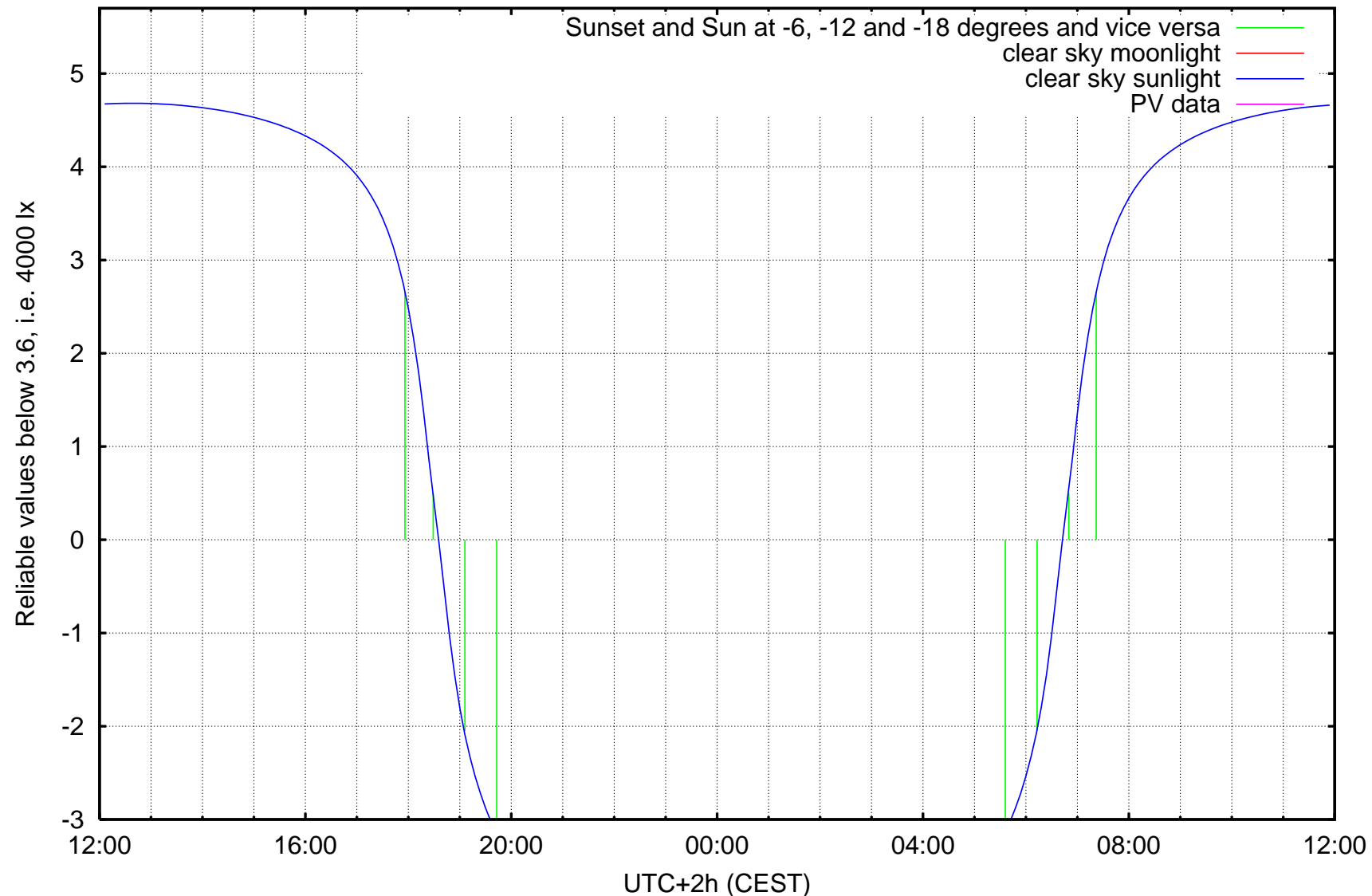
log10 ( illuminance / 1 lx ) Kravi hora, Brno, ending at Friday 2006-10-20 noon
