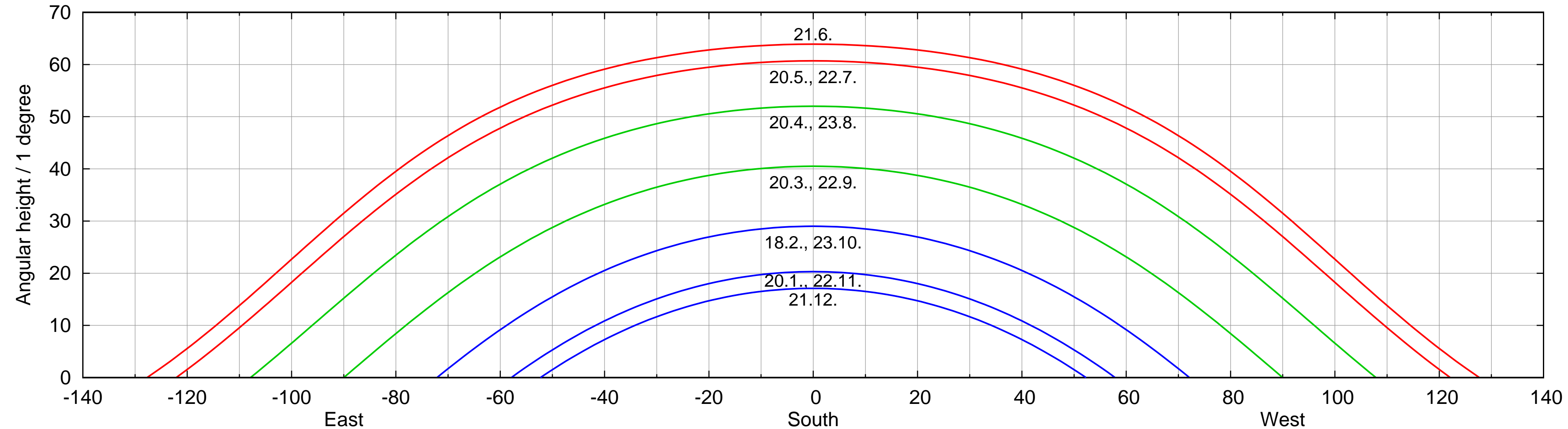
Path of the Sun at 50 degrees latitude (like in Prague)
