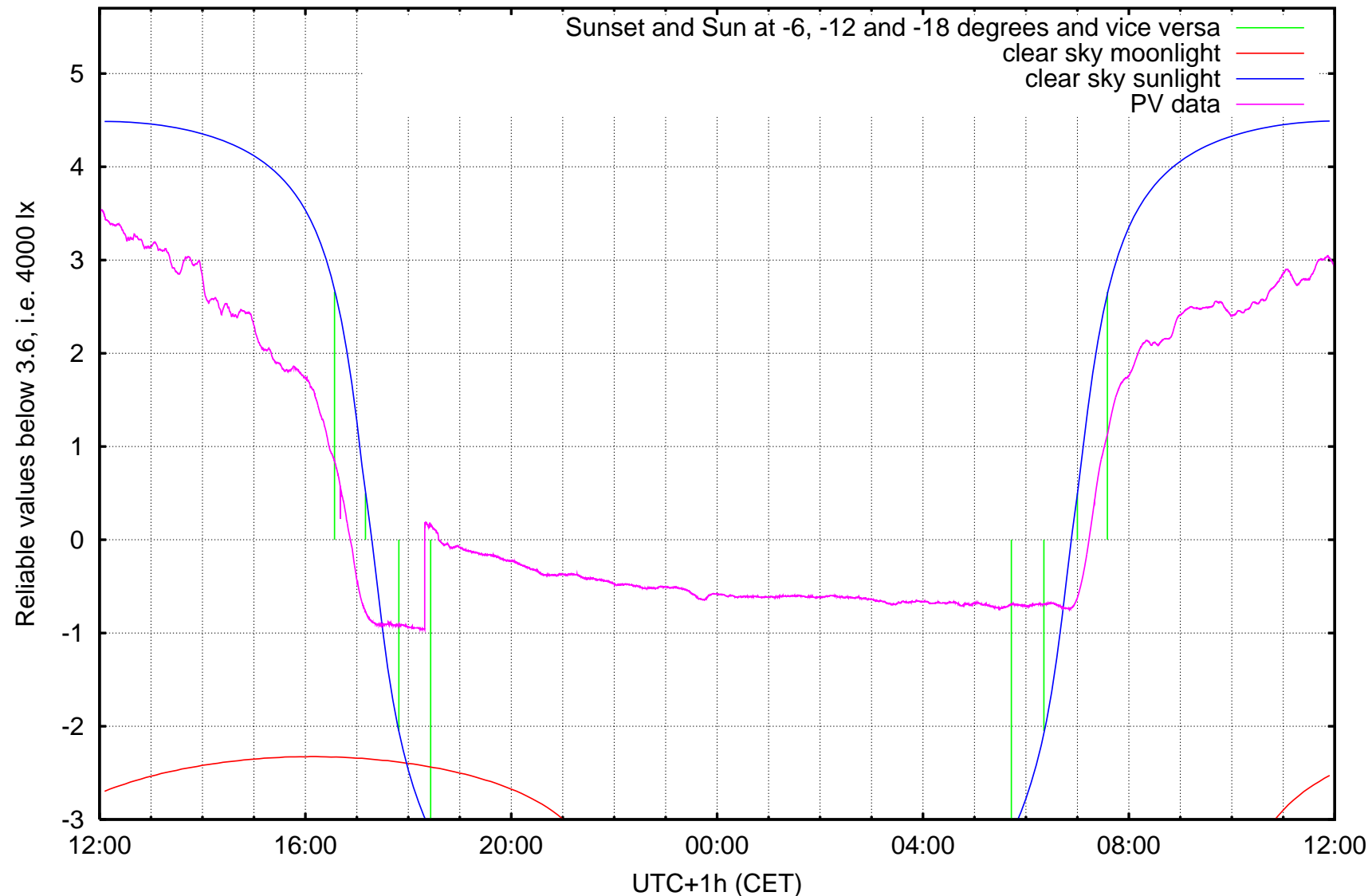
log10 ( illuminance / 1 lx ) Kravi hora, Brno, ending at Wednesday 2007-01-24 noon
