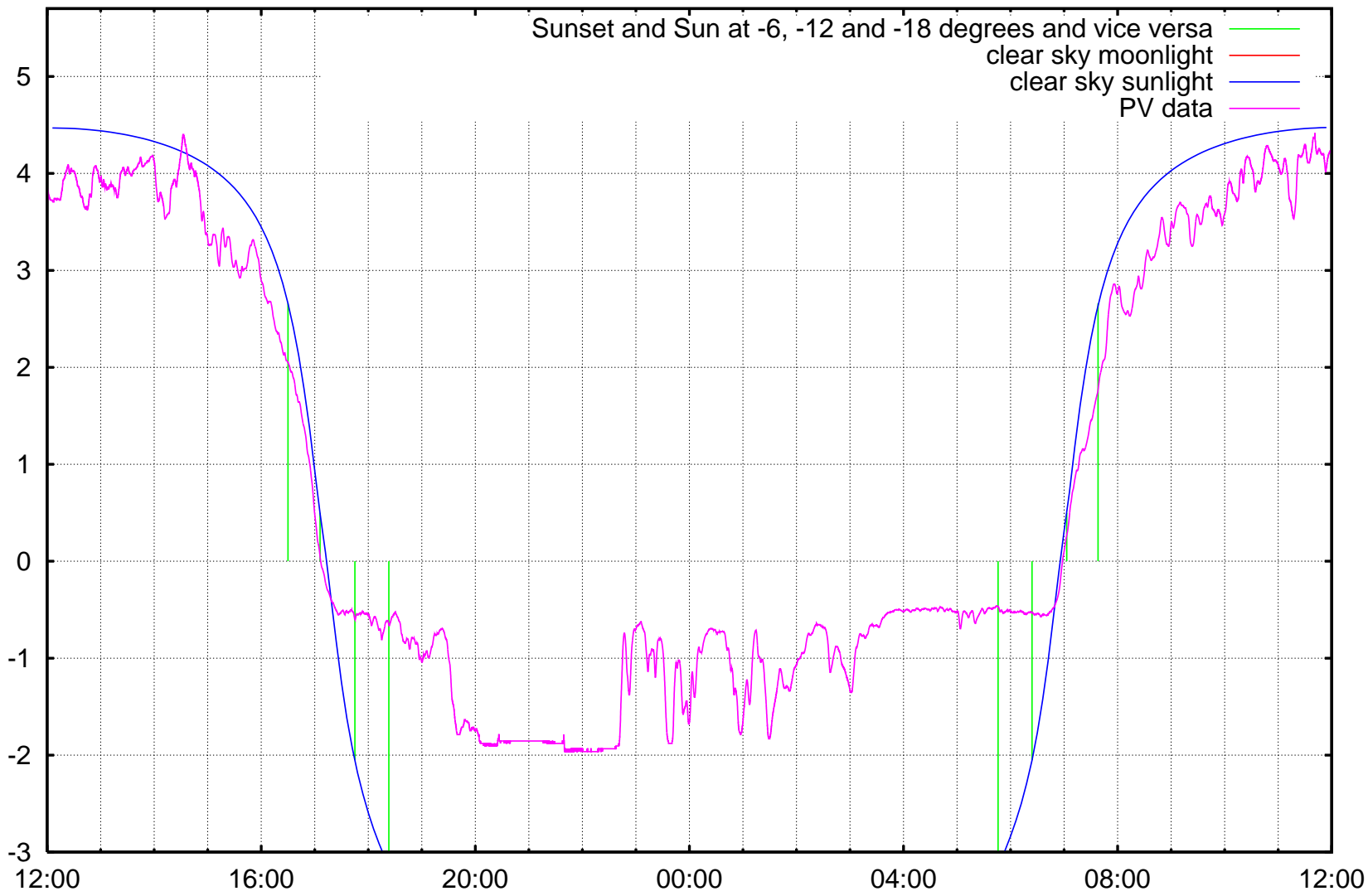
log10 ( illuminance / 1 lx ) Kravi hora, Brno, ending at Sunday 2007-01-21 noon
