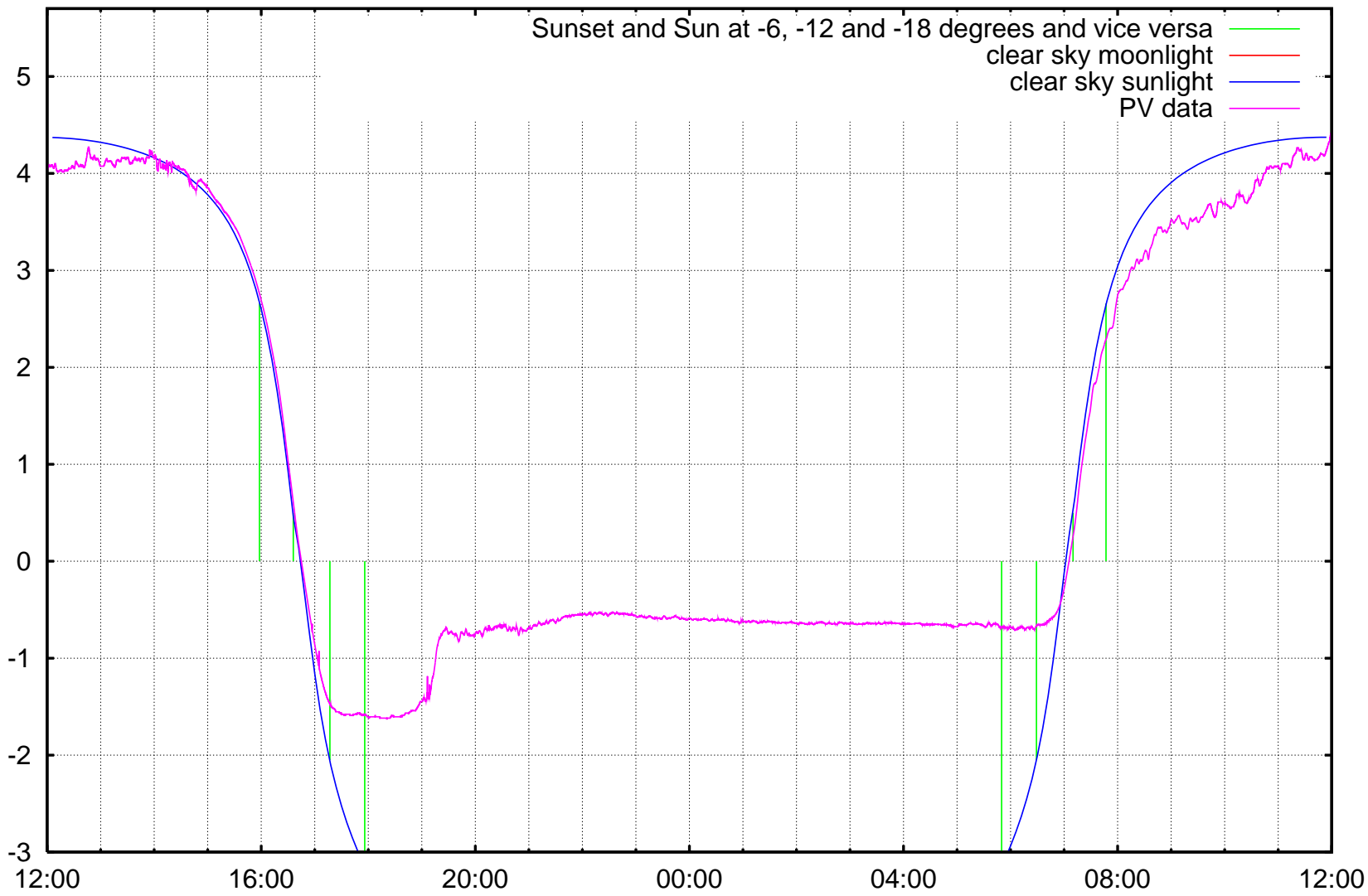
log10 ( illuminance / 1 lx ) Kravi hora, Brno, ending at Sunday 2006-12-24 noon
