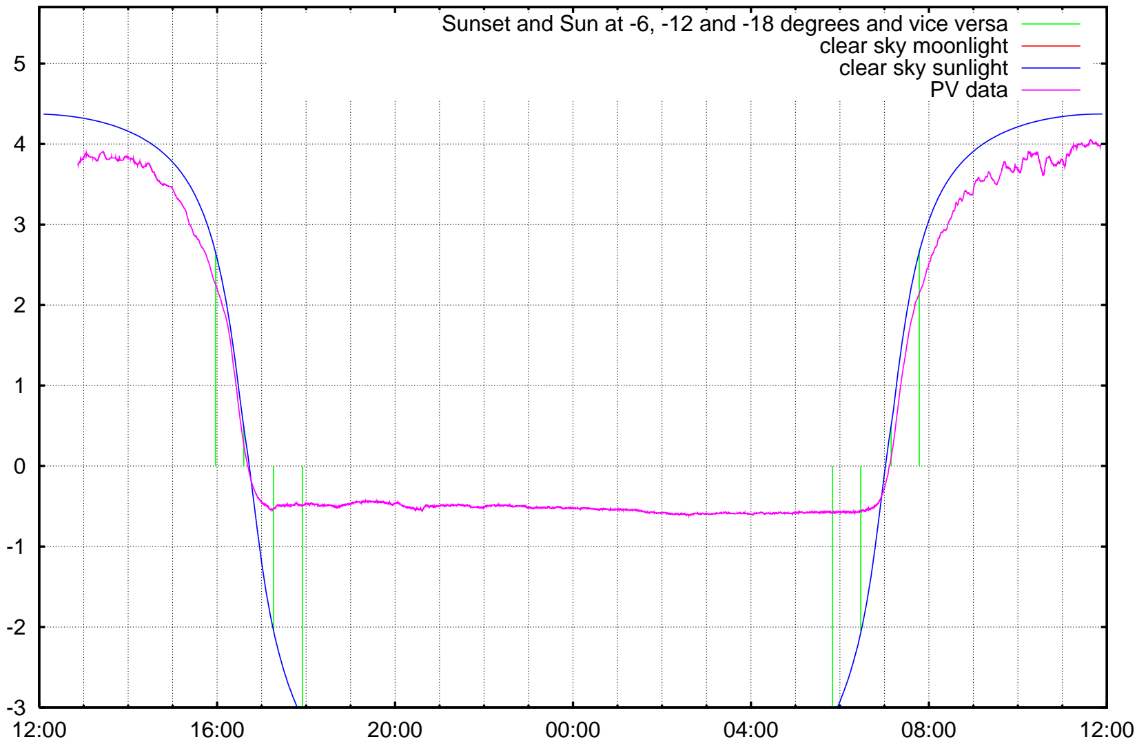
log10 ( illuminance / 1 lx ) Kravi hora, Brno, ending at Saturday 2006-12-23 noon
