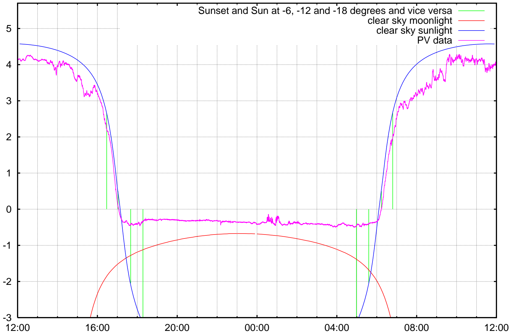
log10 ( illuminance / 1 lx ) Kravi hora, Brno, ending at Sunday 2006-11-05 noon
