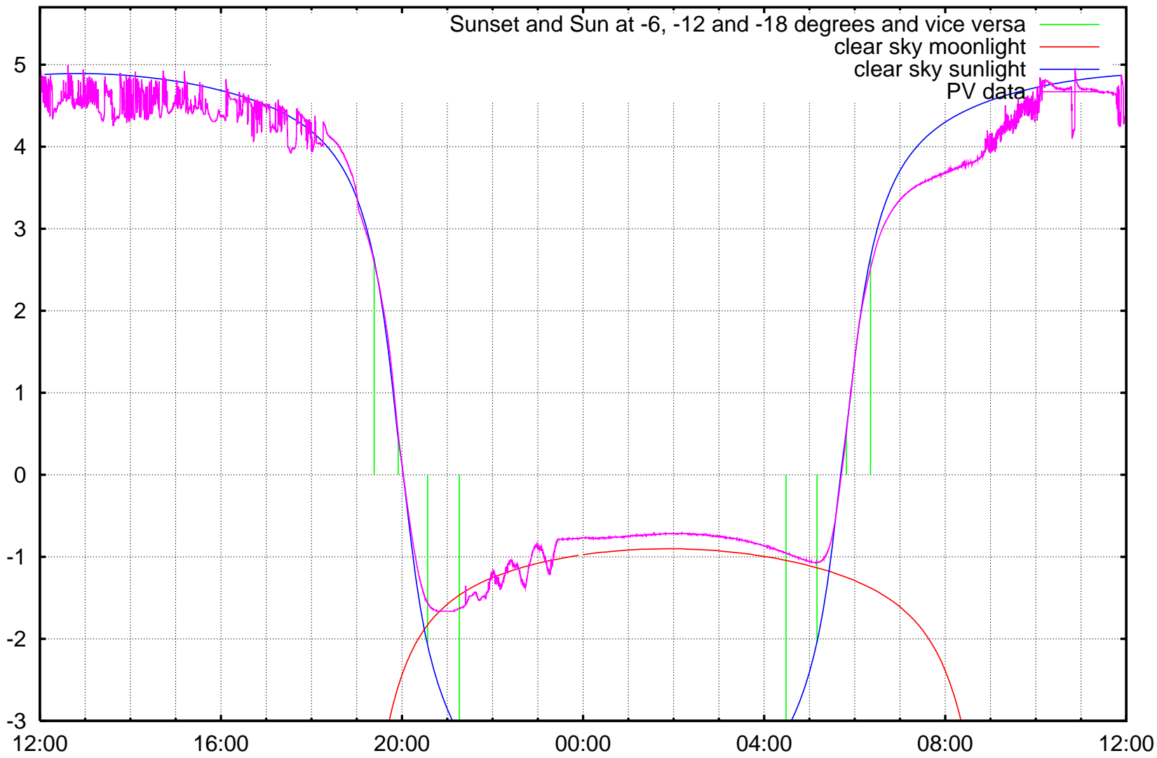
log10 ( illuminance / 1 lx ) Kravi hora, Brno, ending at Saturday 2006-09-09 noon
