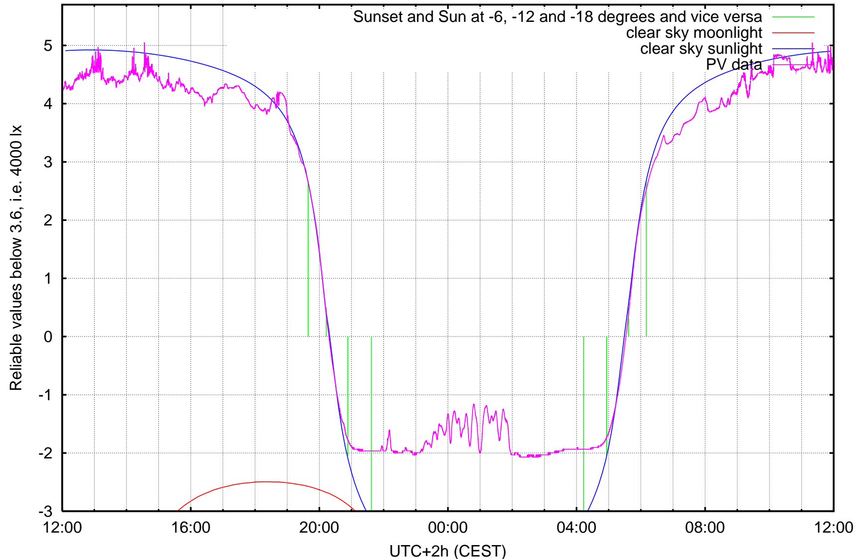
log10 ( illuminance / 1 lx ) Kravi hora, Brno, ending at Friday 2006-09-01 noon
