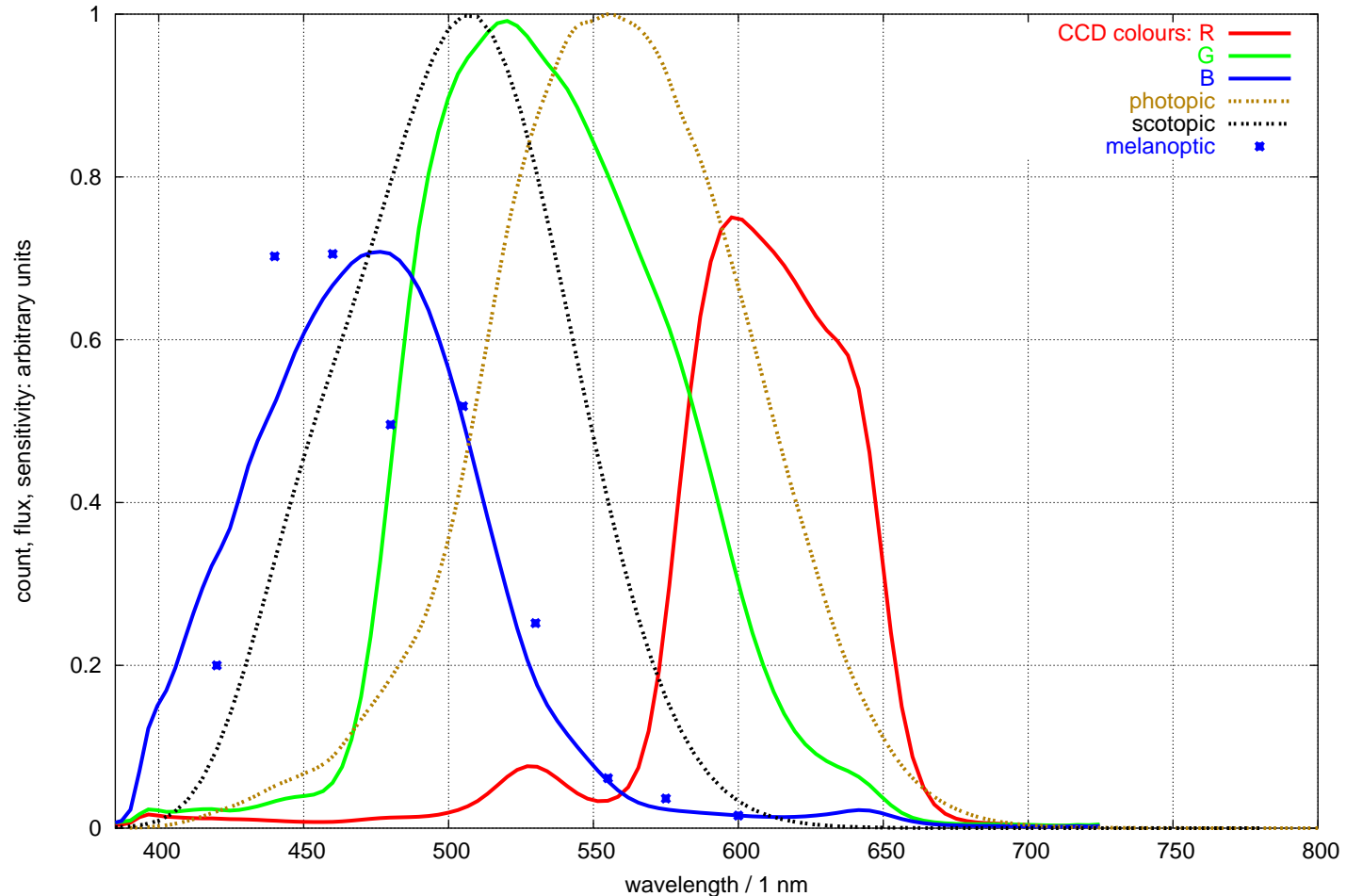
Fuji S5000 spectral sensitivity (preliminary)
