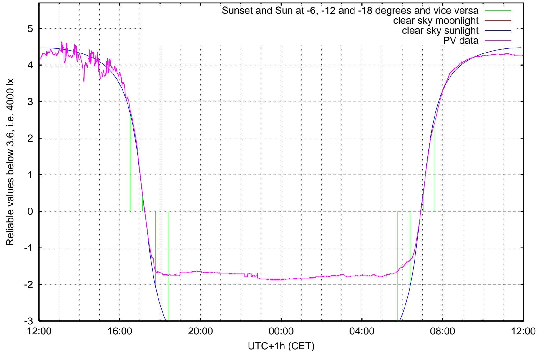
log10 ( illuminance / 1 lx ) Kravi hora, Brno, ending at Monday 2007-01-22 noon
