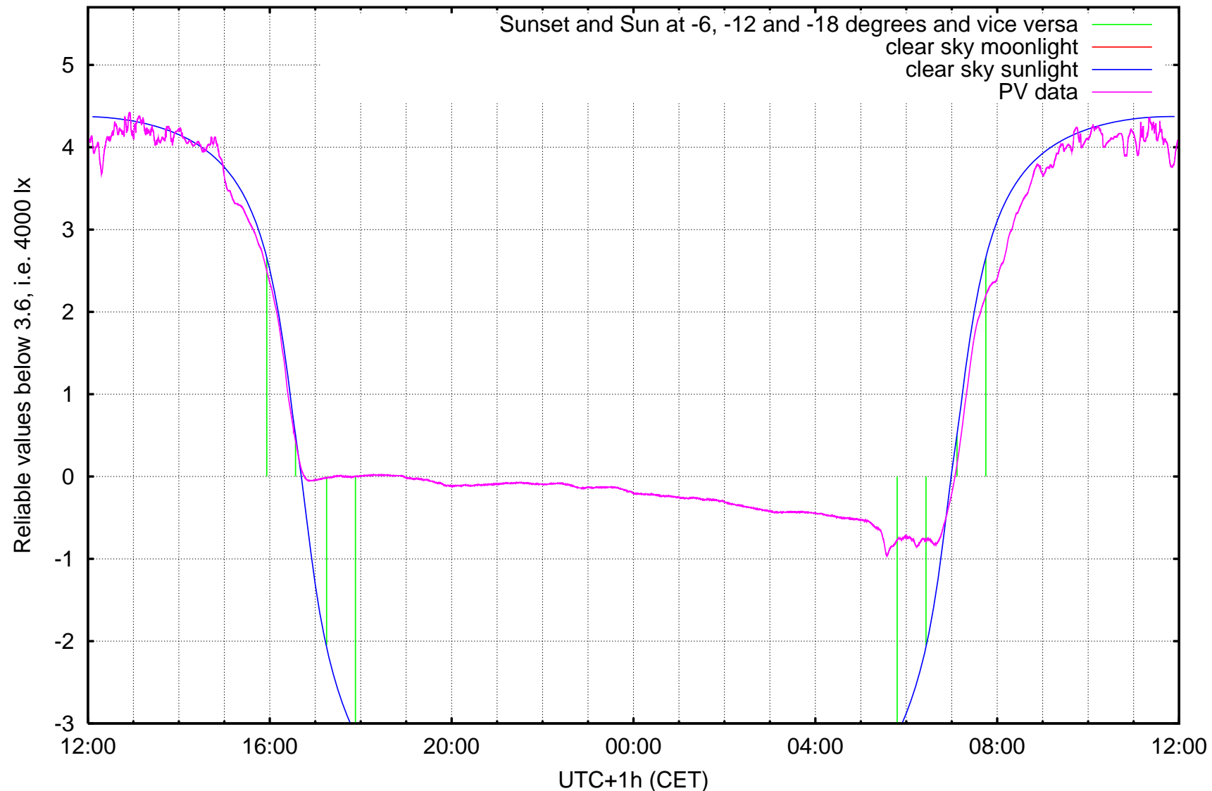
log10 ( illuminance / 1 lx ) Kravi hora, Brno, ending at Tuesday 2006-12-19 noon
