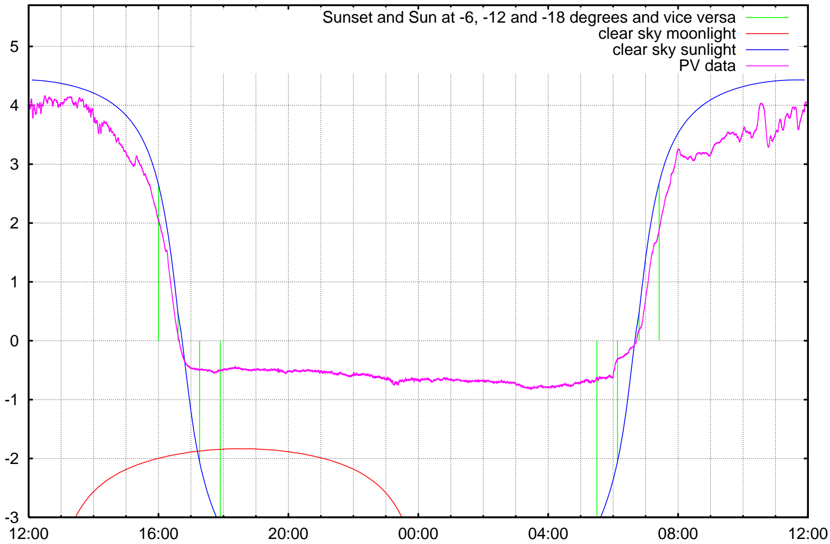
log 10 ( illuminance / 1 lx ) Kravi hora, Brno, ending at Wednesday 2006-11-29 noon
