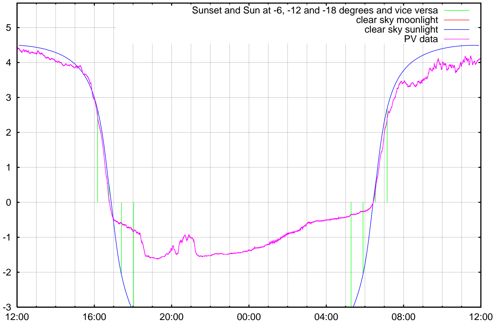
log10 ( illuminance / 1 lx ) Kravi hora, Brno, ending at Saturday 2006-11-18 noon
