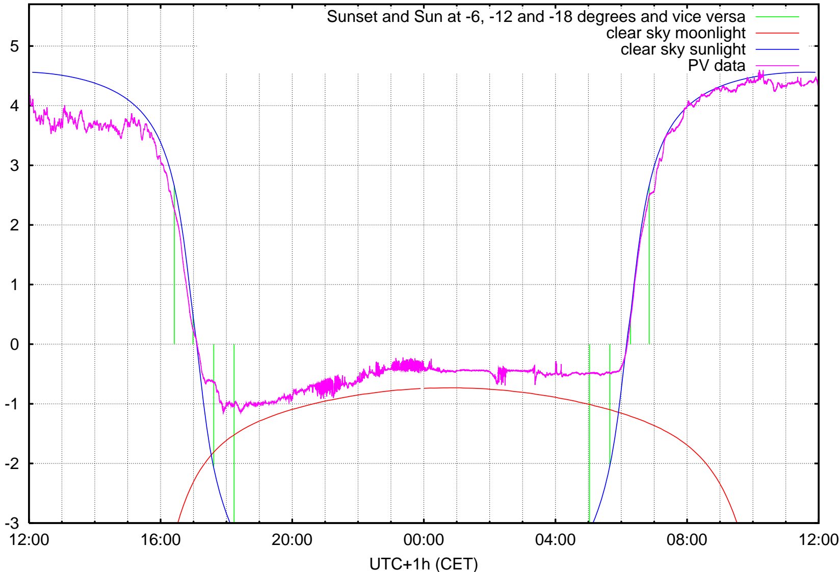
log10 ( illuminance / 1 lx ) Kravi hora, Brno, ending at Tuesday 2006-11-07 noon
