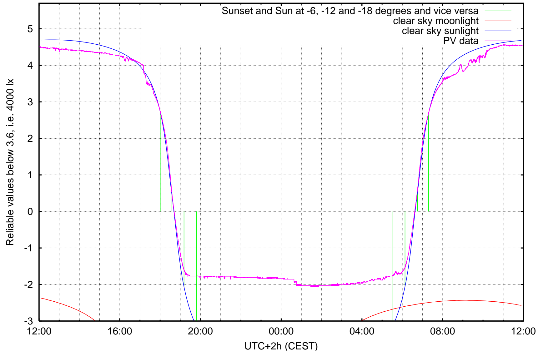
log10 ( illuminance / 1 lx ) Kravi hora, Brno, ending at Tuesday 2006-10-17 noon
