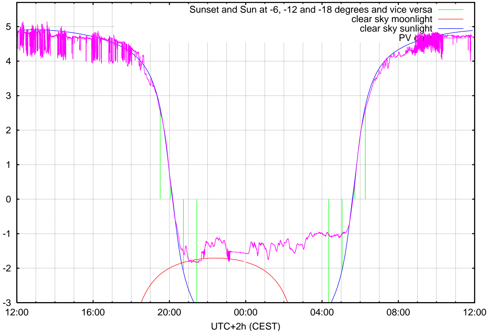
log10 ( illuminance / 1 lx ) Kravi hora, Brno, ending at Tuesday 2006-09-05 noon
