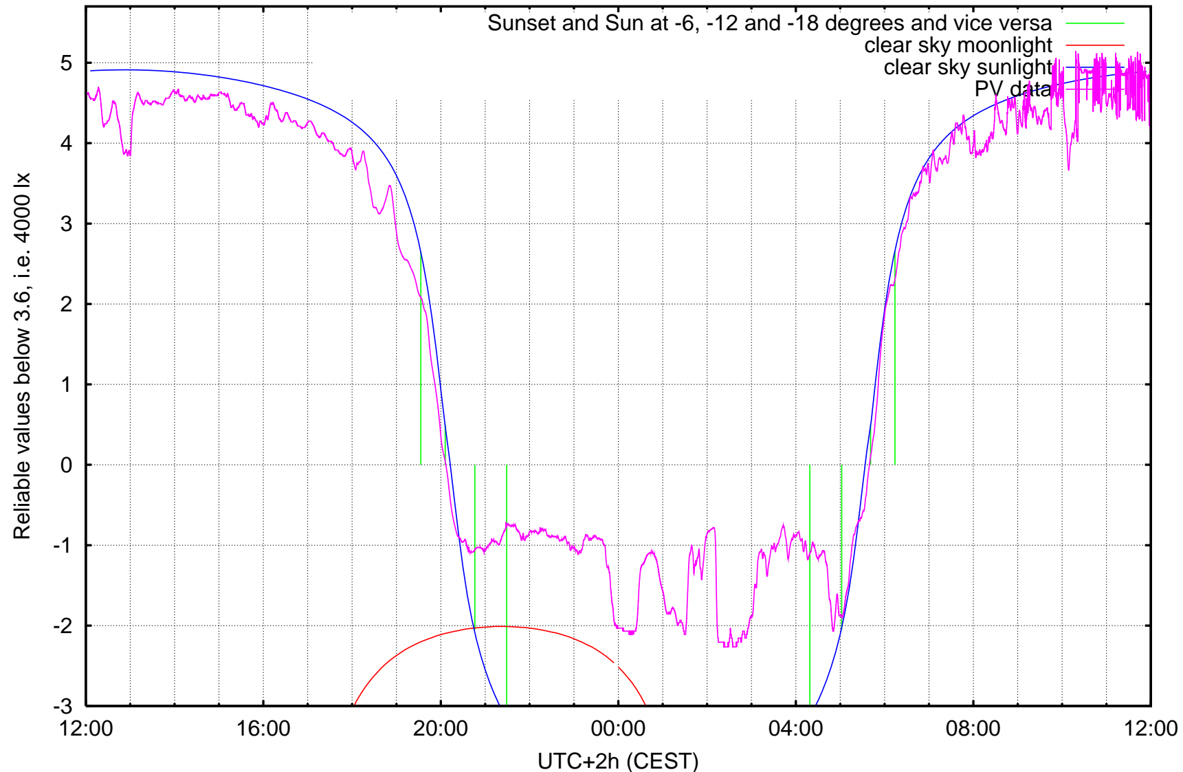
log10 ( illuminance / 1 lx ) Kravi hora, Brno, ending at Monday 2006-09-04 noon
