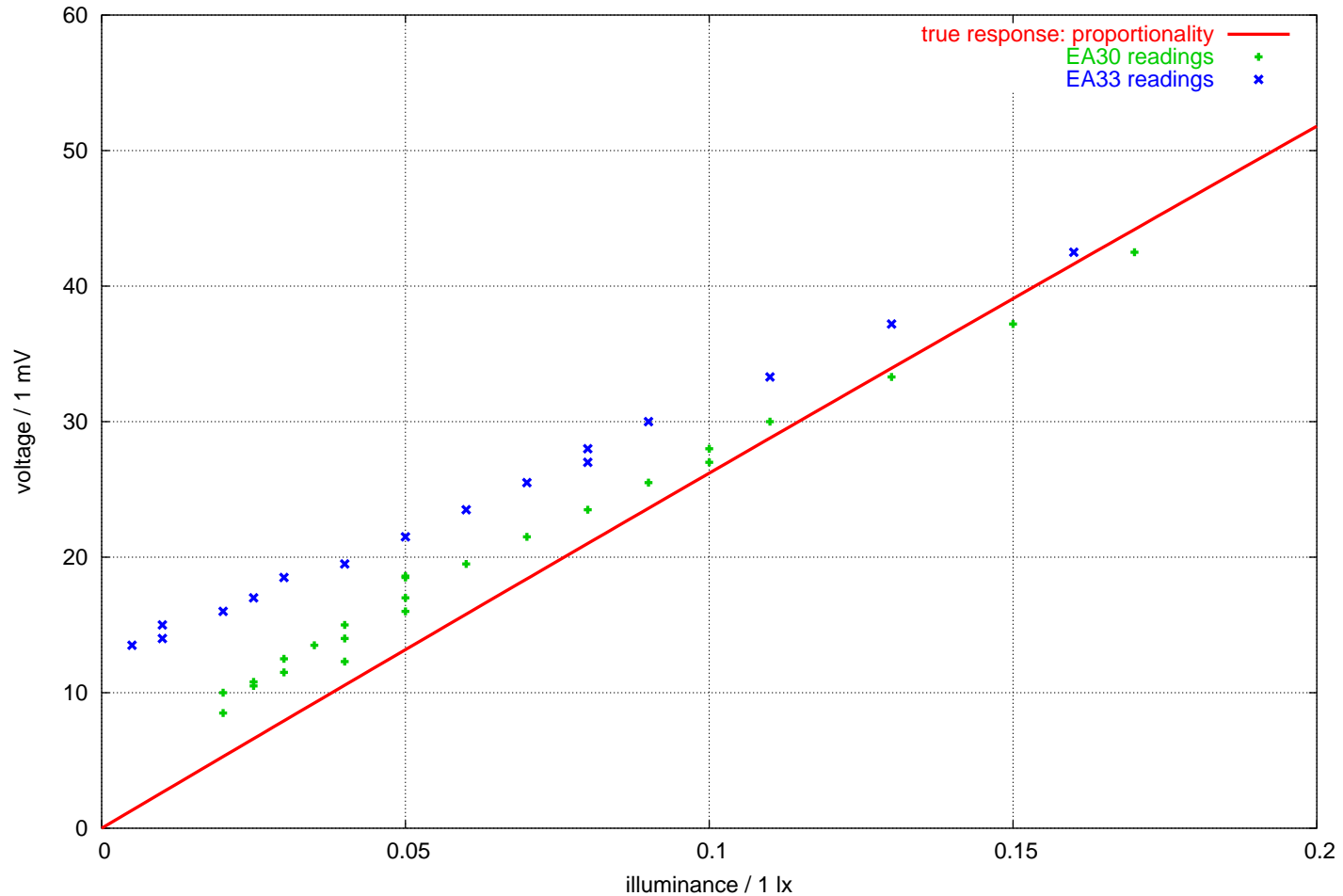
Solar panel voltage at various illuminations
