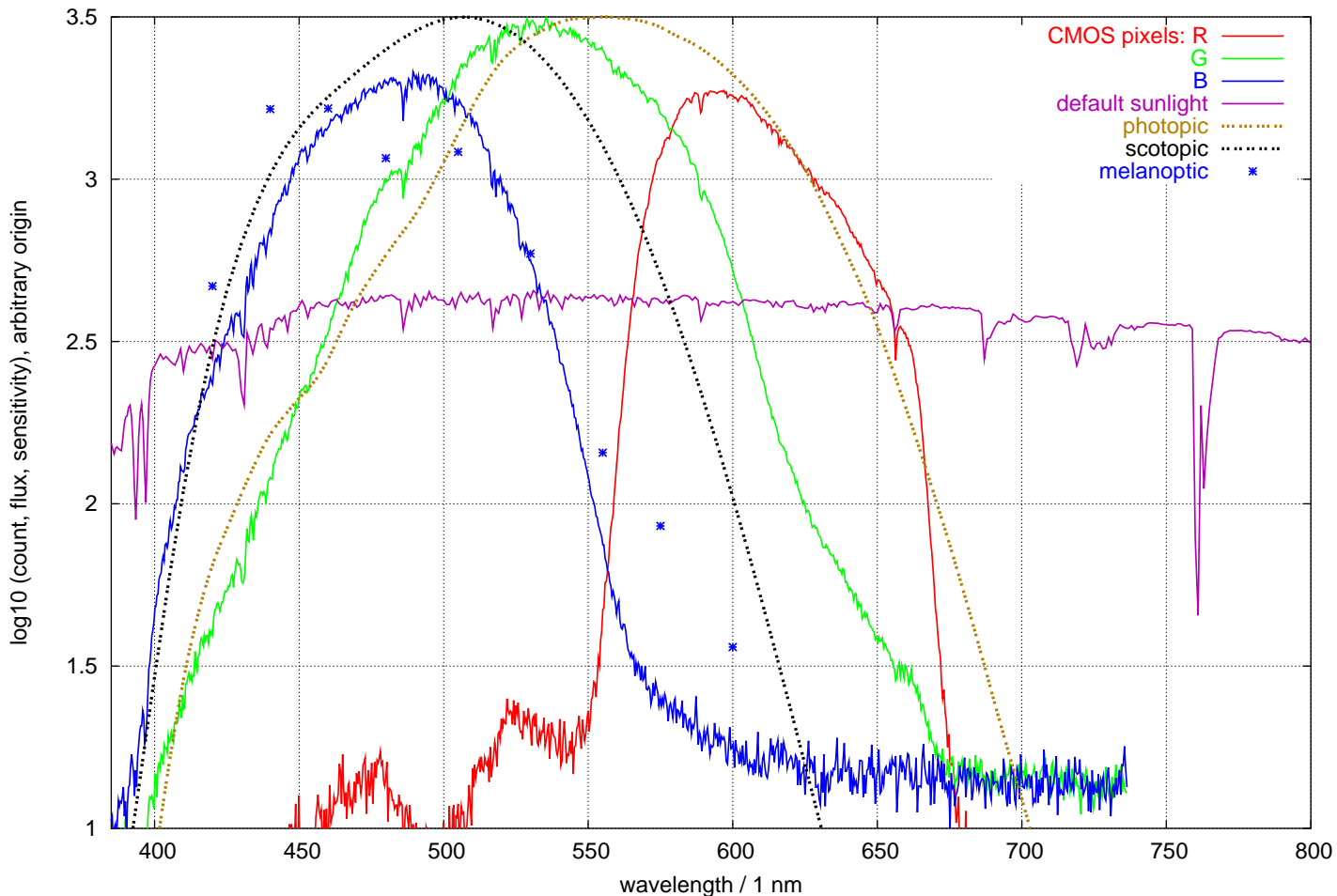
Canon EOS D60 raw solar spectrum at airmass=1.33
