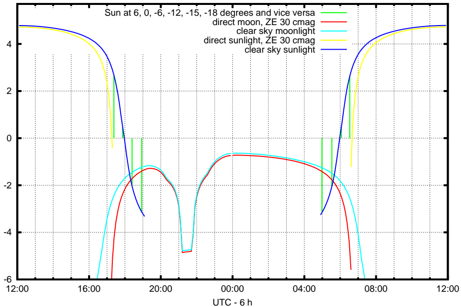
log 10 ( illuminance / 1 lx ) at Mishawaka ending at Thursday 2008-02-21 noon
