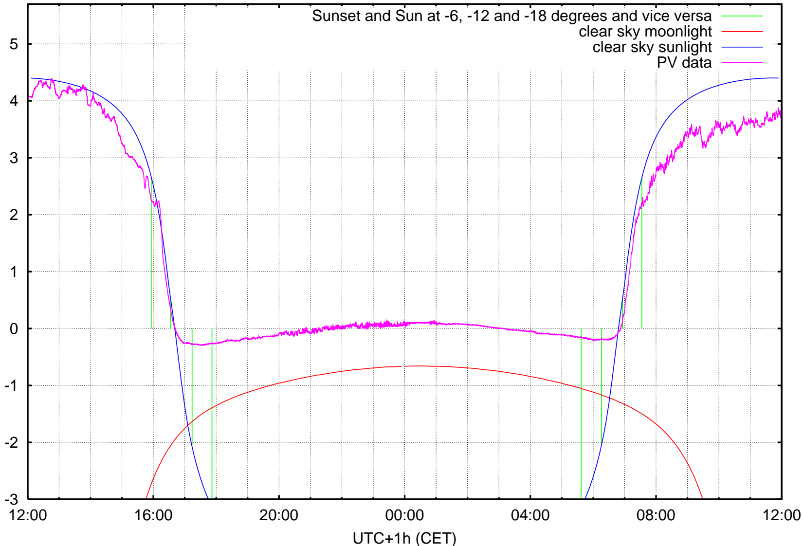
log10 ( illuminance / 1 lx ) Kravi hora, Brno, ending at Wednesday 2006-12-06 noon
