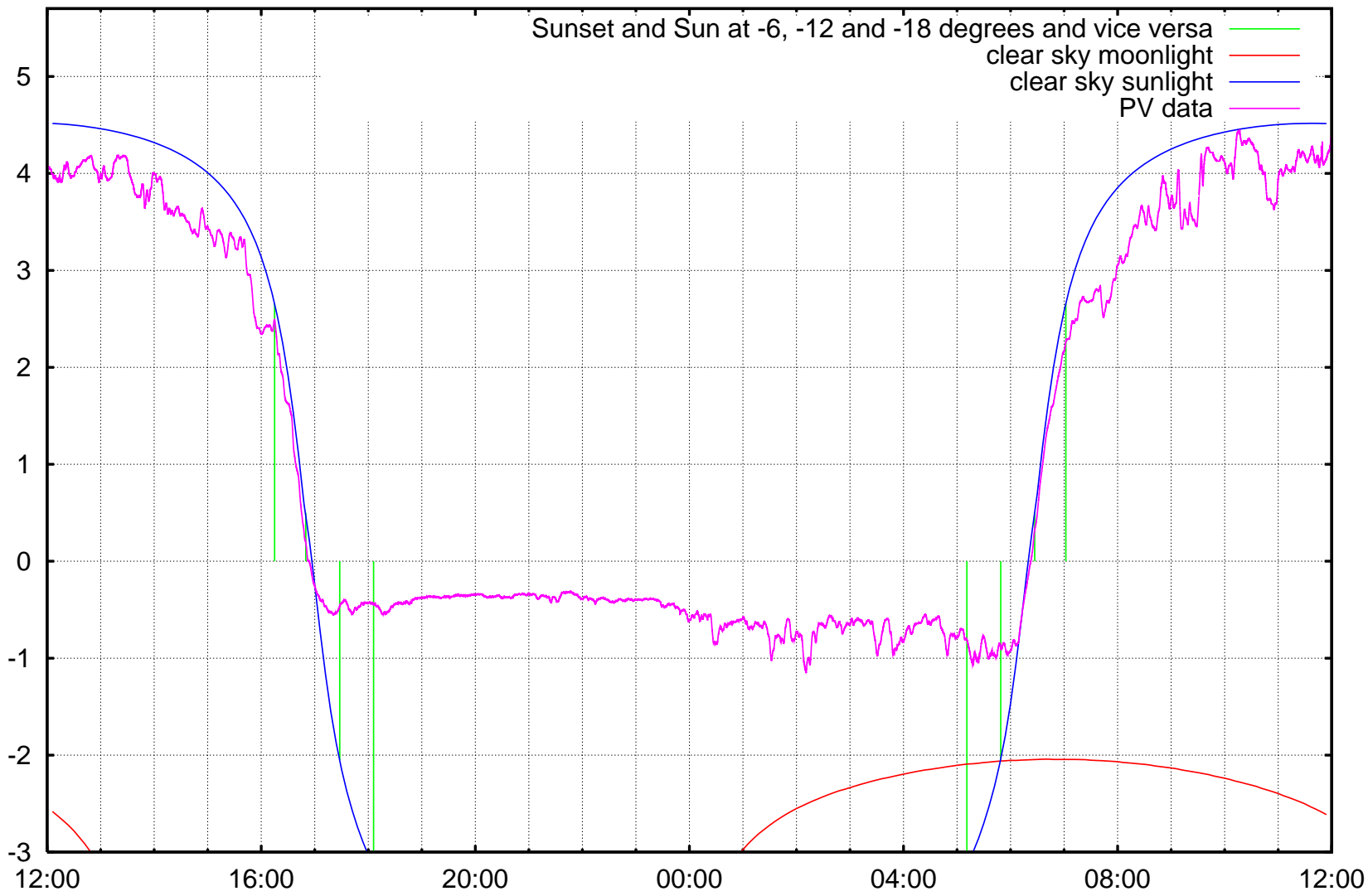
log10 ( illuminance / 1 lx ) Kravi hora, Brno, ending at Tuesday 2006-11-14 noon
