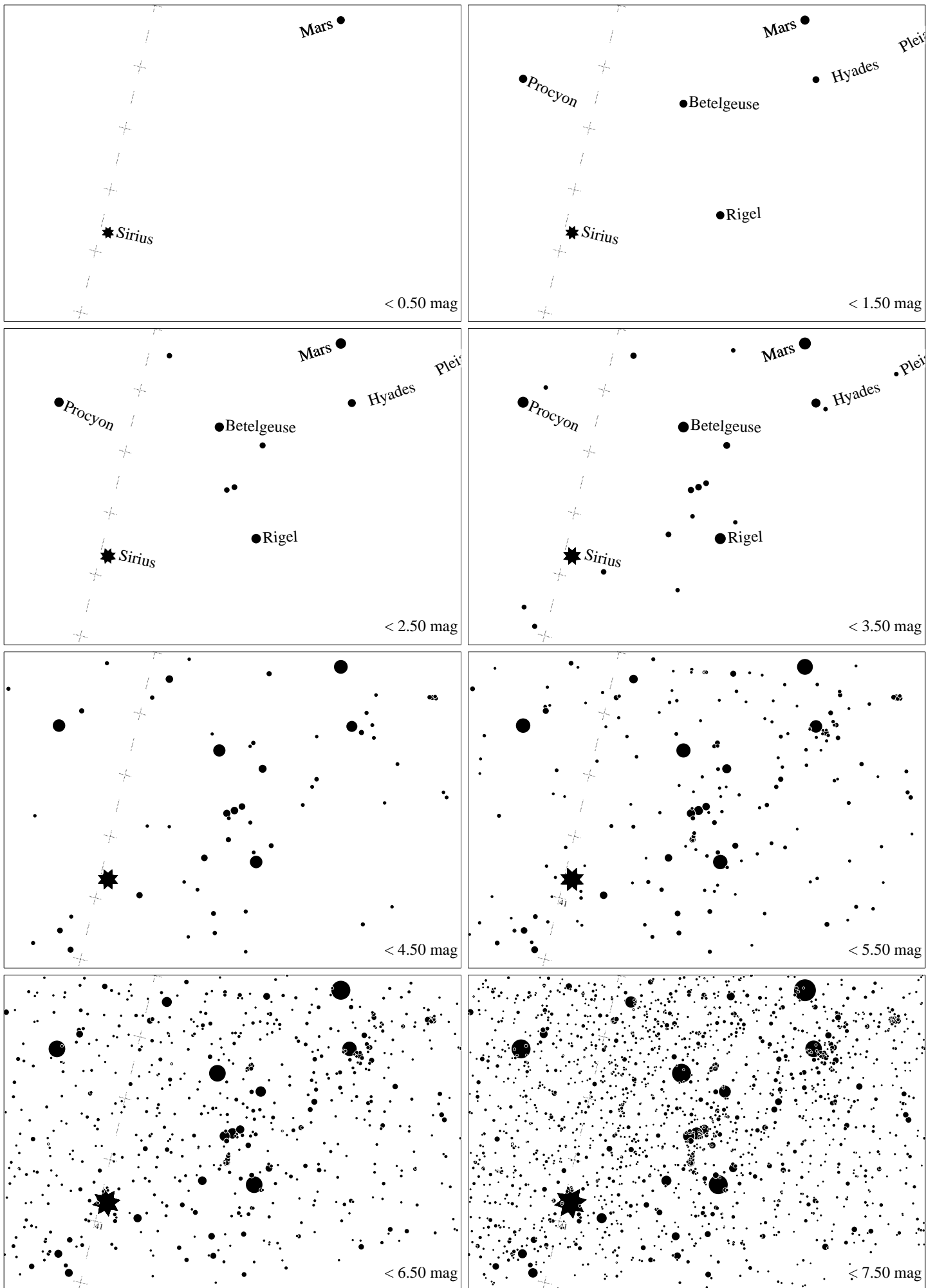
Maps for Globe at Night at latitude 50^\circ , 2023-02-17, 21:00 local time (Sun at -35^\circ ), transparent air. Lines from N(E,S,W) to zenith shown (crosses each 10^\circ ). Orion 's belt is 23^\circ to the right from S, at 36^\circ height. Star clusters M 41 and M35 marked when appropriate. Map vertical size is 50^\circ . Jan Hollan maps, CzechGlobe
