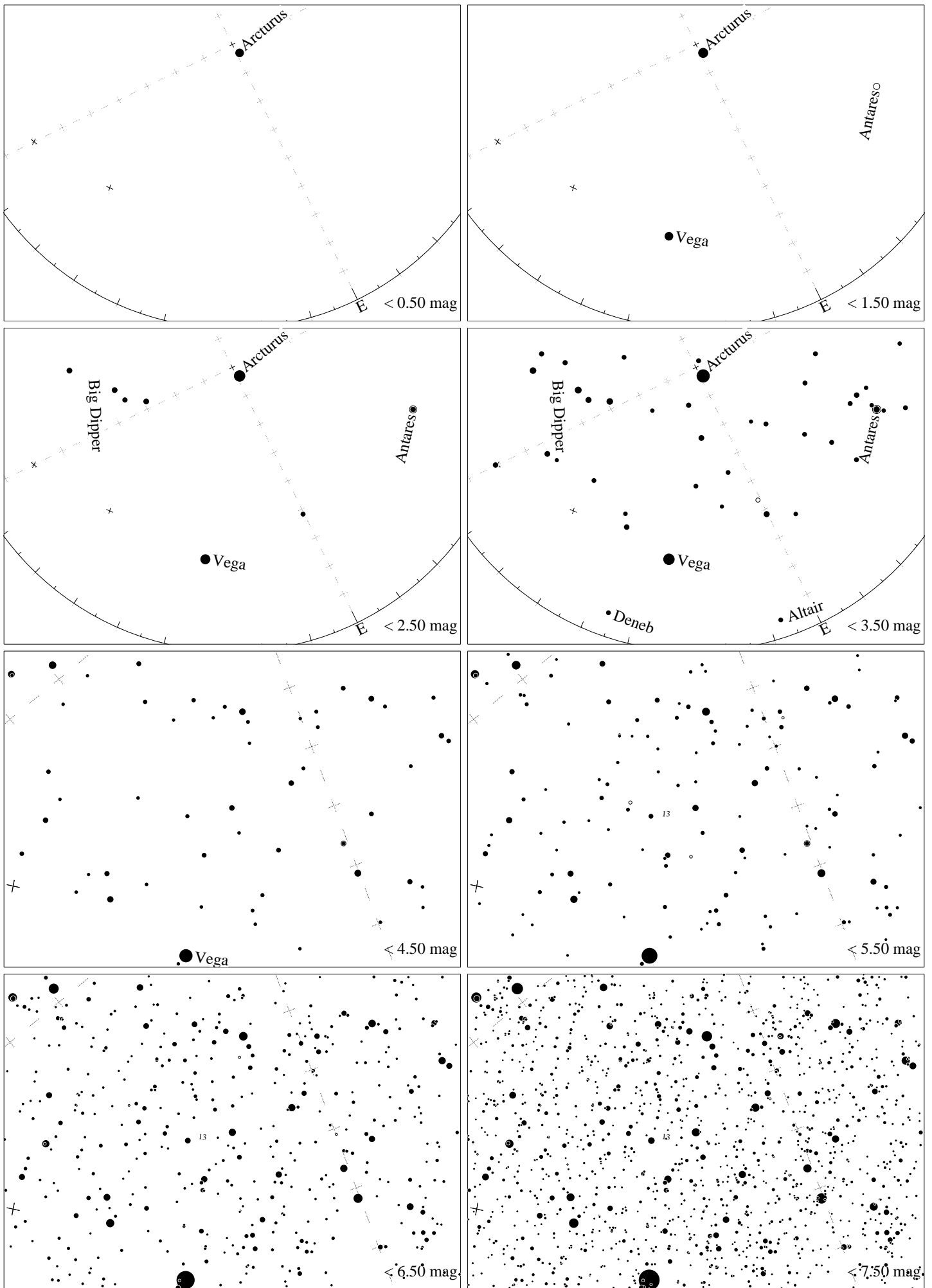
Maps for Globe at Night latitude 20^\circ , 2021-06-06, 21 h local time (Sun at -29^\circ ), transparent air. Lines from N(E,S,W) to zenith shown (crosses each 10^\circ ). Centered on \zeta Herculis, which is 64^\circ to the right from N, at 52^\circ height. Detailed maps 50^\circ vertically, the first four maps 100^\circ . Jan Hollan, CzechGlobe
