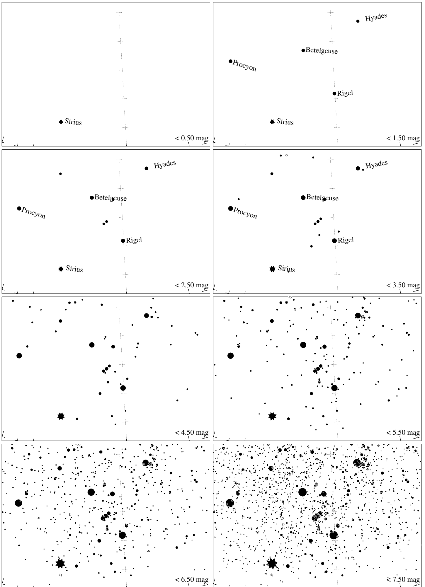
Maps for Globe at Night at latitude 60^\circ , 2017-01-23, 21 h local time (Sun at -37^\circ ), transparent air. Lines from N(E,S,W) to zenith shown (crosses each 10^\circ ). Orion's belt is 7^\circ to the left from S, at 29^\circ height. Star clusters M 41 and M35 marked when appropriate. Map vertical size is 50^\circ . Jan Hollan, CzechGlobe
