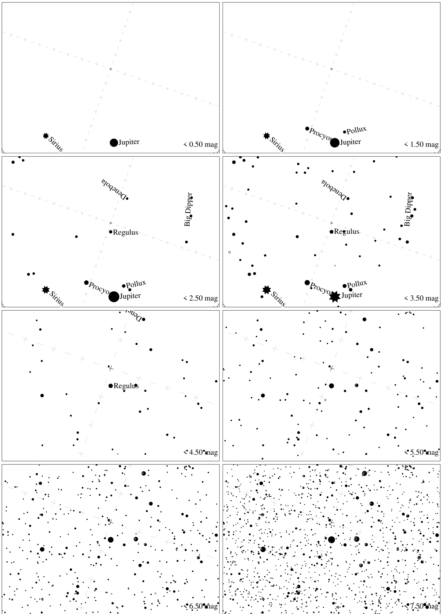
Maps for Globe at Night at latitude 10^\circ , 2026-04-14, 21 h local time (Sun at -41^\circ ), transparent air. Lines from N(E,S,W) to zenith shown (crosses each 10^\circ ). Regulus ( \alpha Leonis) is 71^\circ to the left from N, at 84^\circ height. Detailed maps 50^\circ vertically, the first four maps 100^\circ . Jan Hollan maps, CzechGlobe
