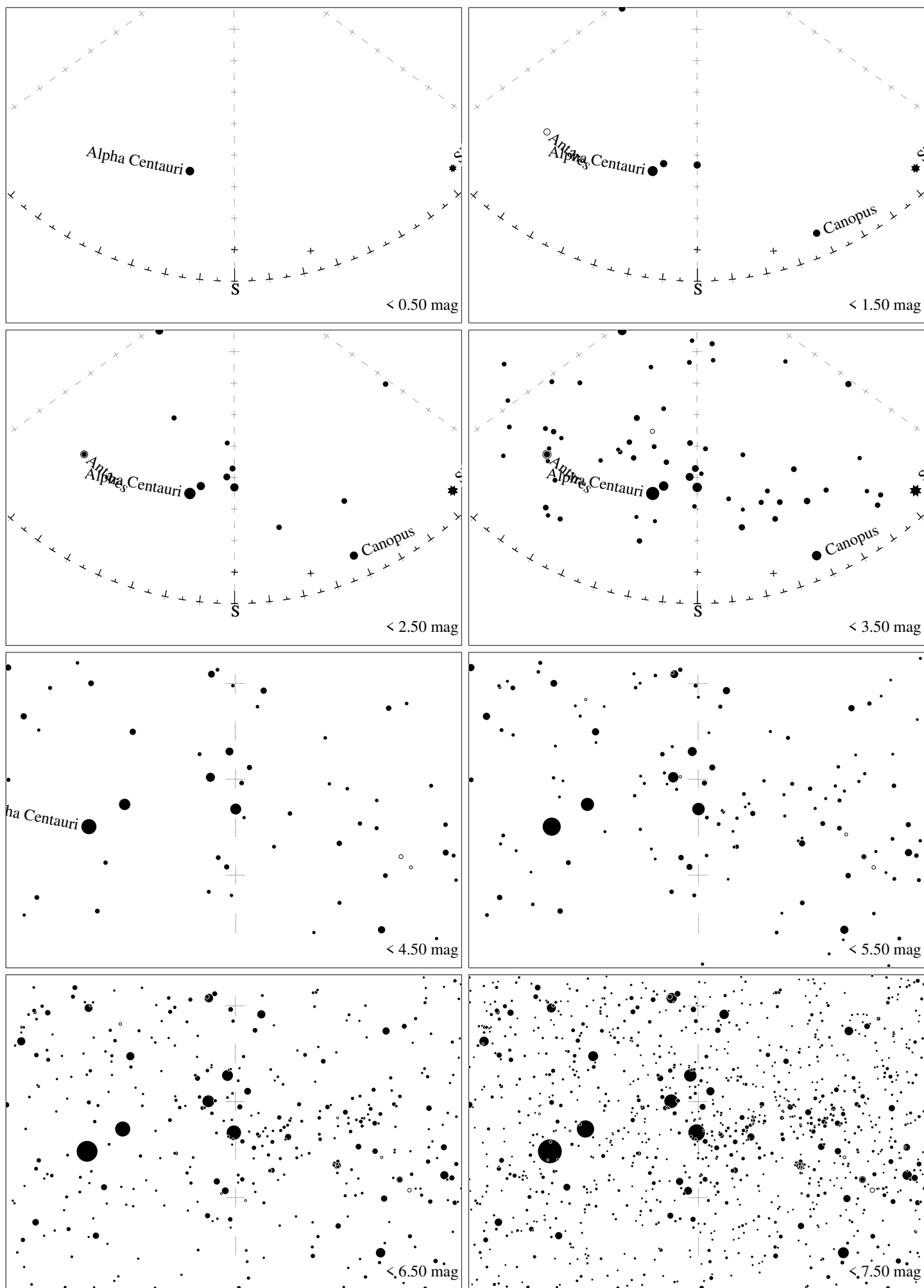
Maps for Globe at Night latitude -10^\circ , 2026-05-13, 21 h local time (Sun at -46^\circ ), transparent air. Central star Acrux (the brightest one in the Cross) is 0^\circ left from the south, at 37^\circ height. Detailed maps 33^\circ vertically, the first four maps 100^\circ . Jan Hollan, CzechGlobe
