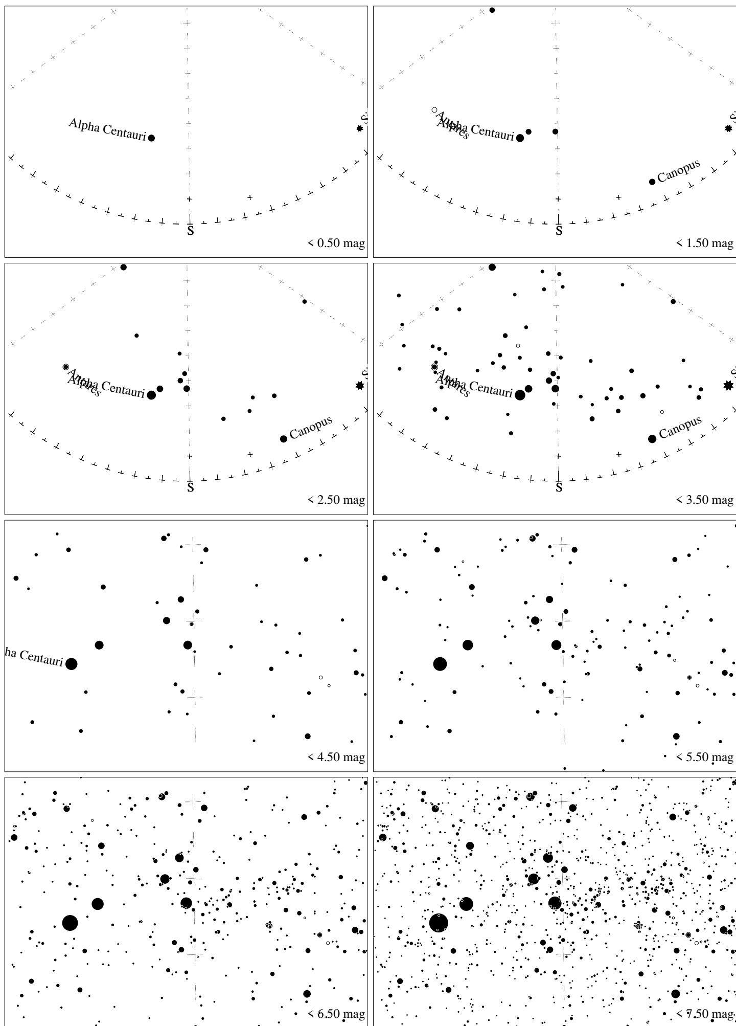
Maps for Globe at Night latitude -10^\circ , 2026-05-11, 21 h local time (Sun at -47^\circ ), transparent air. Central star Acrux (the brightest one in the Cross) is 1^\circ left from the south, at 37^\circ height. Detailed maps 33^\circ vertically, the first four maps 100^\circ . Jan Hollan, CzechGlobe
