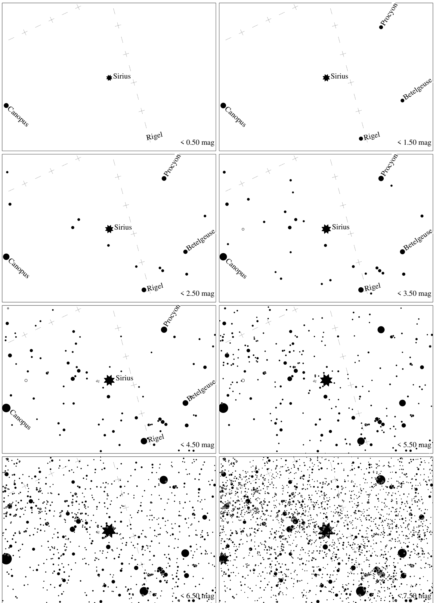
Maps for Globe at Night at latitude -10^\circ , 2026-03-15, 21:00 local time (Sun at -42^\circ ), transparent air. Lines from N(E,S,W) to zenith shown (crosses each 10^\circ ). The brightest fixed star Sirius is 73^\circ to the right from S, at 63^\circ height. Star cluster M 41 marked when appropriate. Map vertical size is 50^\circ . Jan Hollan, CzechGlobe
