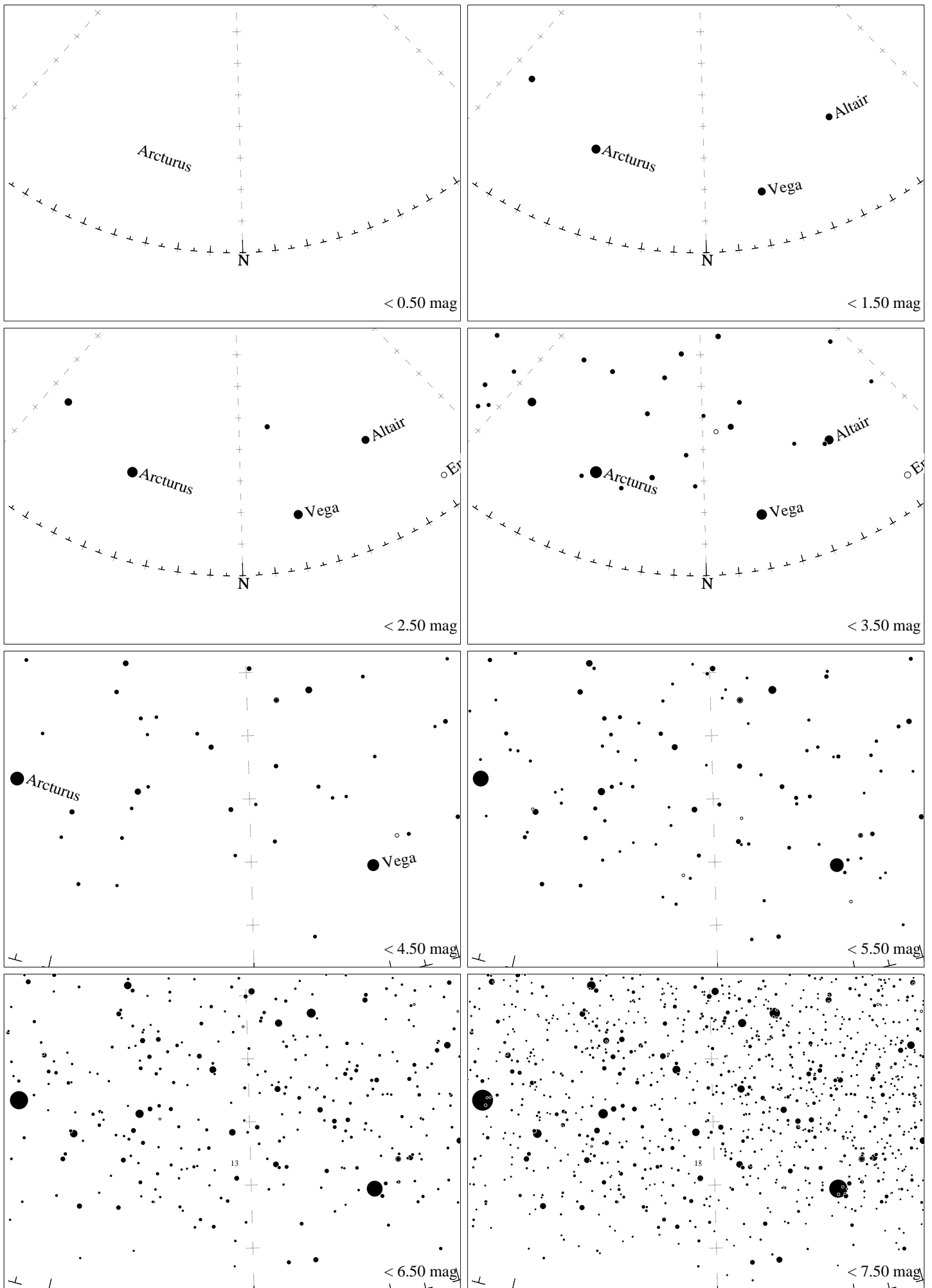
Maps for Globe at Night latitude -30^\circ , 2025-07-20, 21 h local time (Sun at -47^\circ ), transparent air. Lines from N(E,S,W) to zenith shown (crosses each 10^\circ ). Centered on \zeta Herculis, which is 3^\circ to the left from N, at 28^\circ height. Detailed maps 50^\circ vertically, the first four maps 100^\circ . Jan Hollan, CzechGlobe
