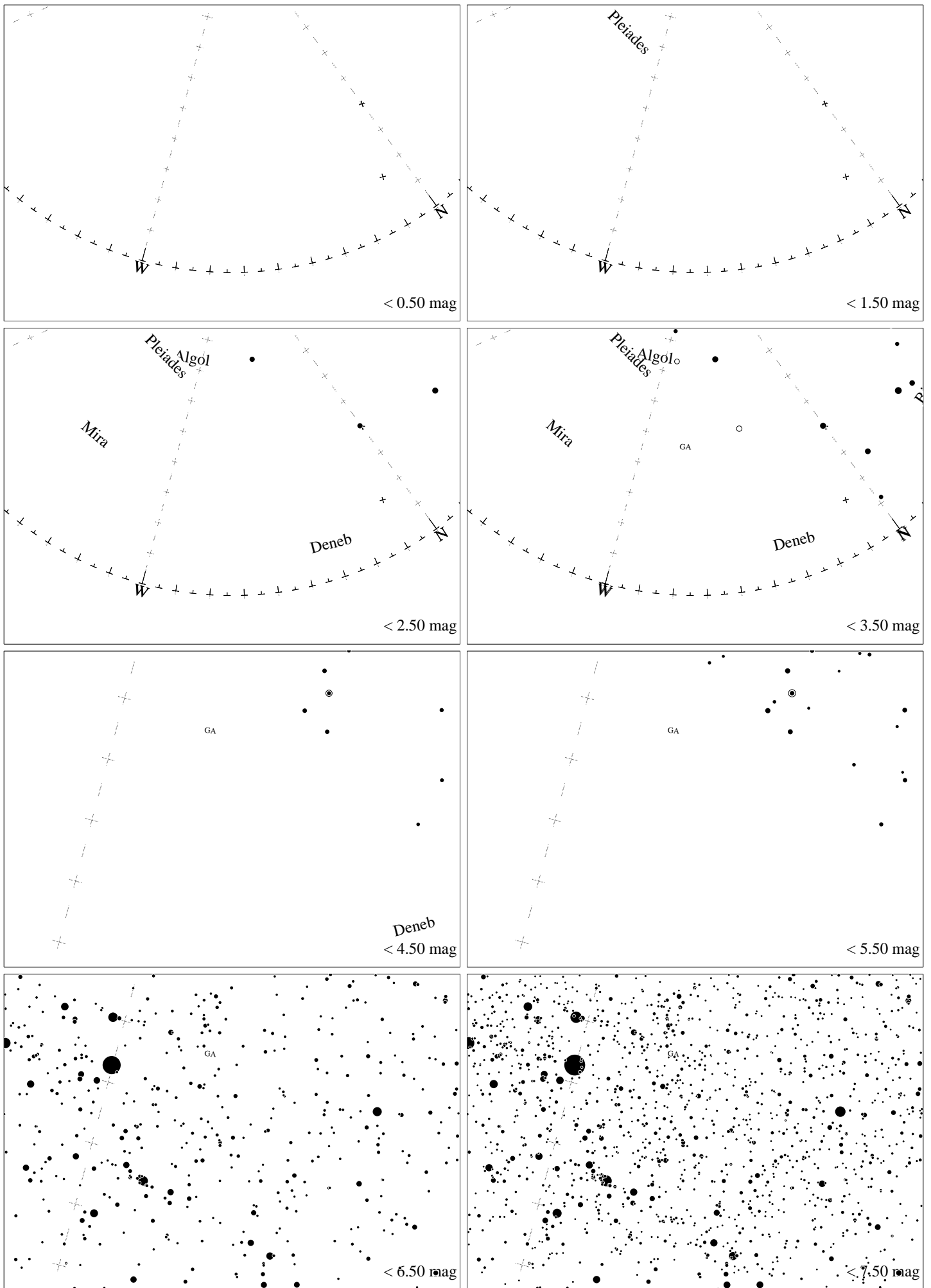
Maps for Globe at Night latitude 40^\circ , 20254-12-26, 21 h local time (Sun at -56^\circ ), transparent air. Lines from N(E,S,W) to zenith shown (crosses each 10^\circ ). The map is centered on Markab ( \alpha Pegasi), which is 64^\circ to the left from N, at 35^\circ height. Detailed maps 50^\circ vertically, the first four maps 100^\circ . Jan Hollan, CzechGlobe
