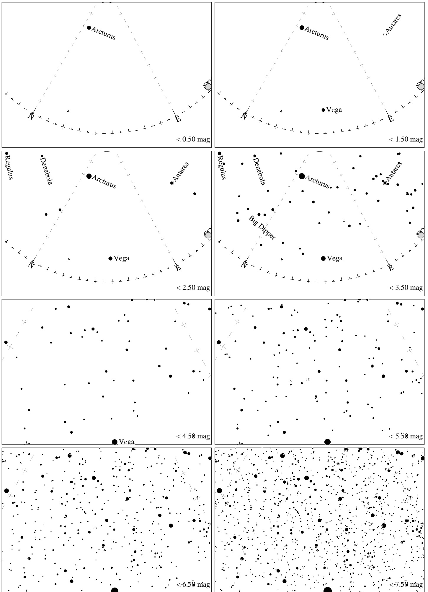
Maps for Globe at Night latitude 0°, 2023-06-06, 21 h local time (Sun at -41^\circ ), transparent air. Lines from N(E,S,W) to zenith shown (crosses each 10^\circ ). Centered on \zeta Herculis, which is 47^\circ to the right from N, at 40^\circ height. Detailed maps 50^\circ vertically, the first four maps 100^\circ . Jan Hollan, CzechGlobe
