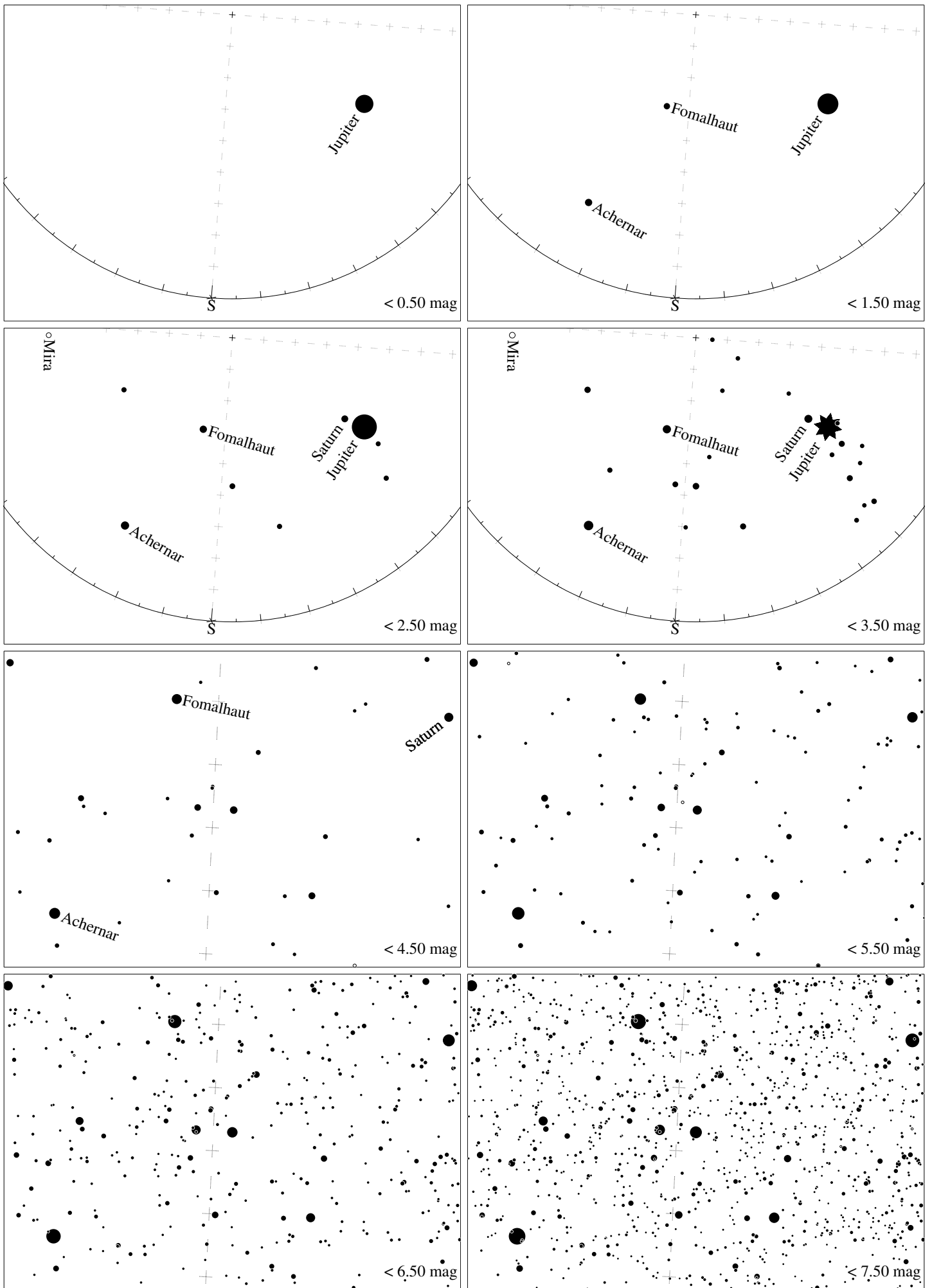
Maps for Globe at Night latitude 0°, 2020-10-12, 21:30 h local time (Sun at -48^\circ ), transparent air. Lines from N(E,S,W) to zenith shown (crosses each 10^\circ ). Centered on Alnair ( \alpha Gruis), which is 4^\circ to the right from S, at 43^\circ height. Detailed maps 50^\circ vertically, the first four maps 100^\circ . Jan Hollan, CzechGlobe
