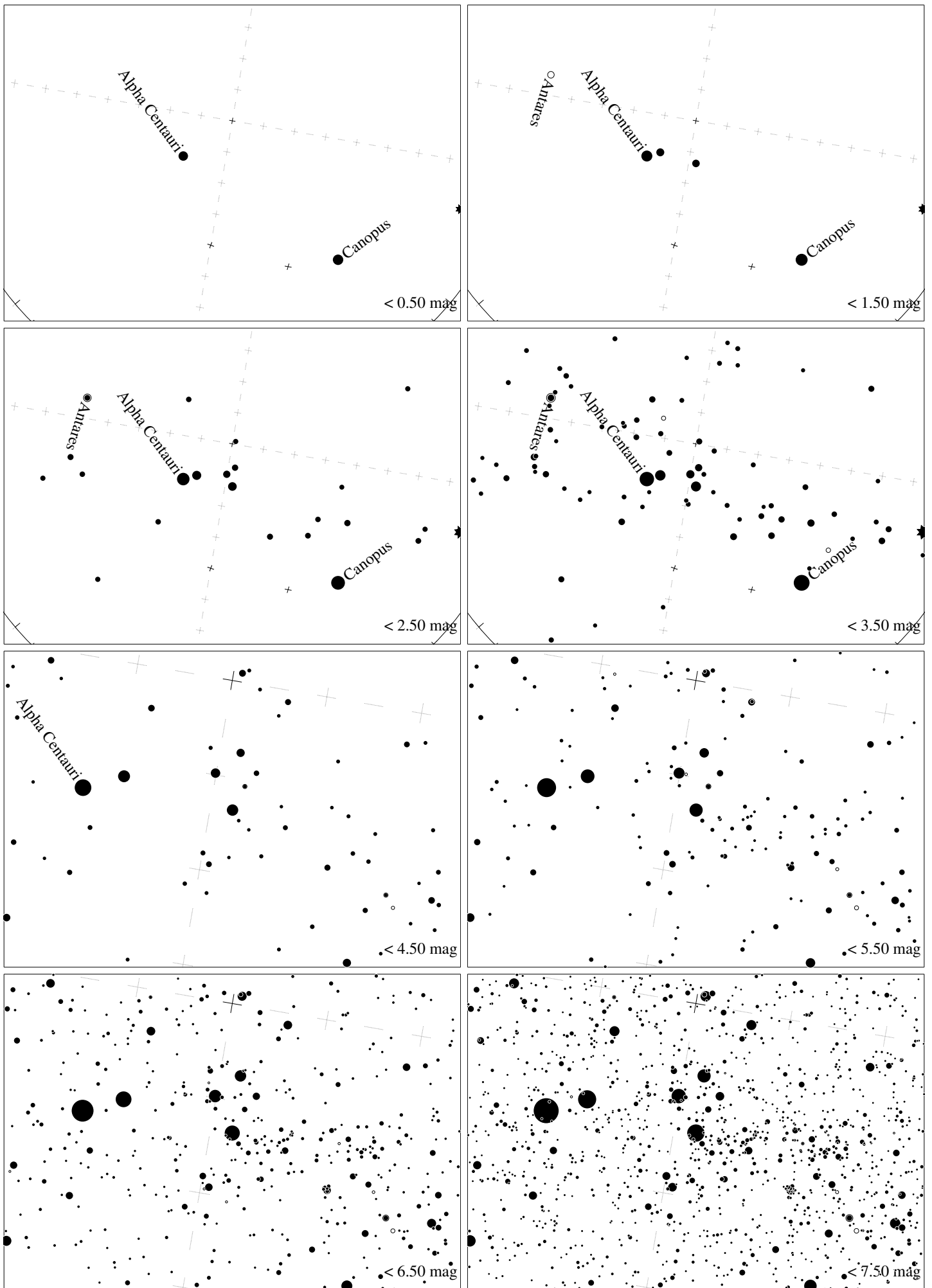
Maps for Globe at Night latitude -50^\circ , 2020-05-18, 21 h local time (Sun at -44^\circ ), transparent air. Central star Acrux (the brightest one in the Cross) is 10^\circ left from the south, at 77^\circ height. Detailed maps 33^\circ vertically, the first four maps 100^\circ . Jan Hollan, CzechGlobe
