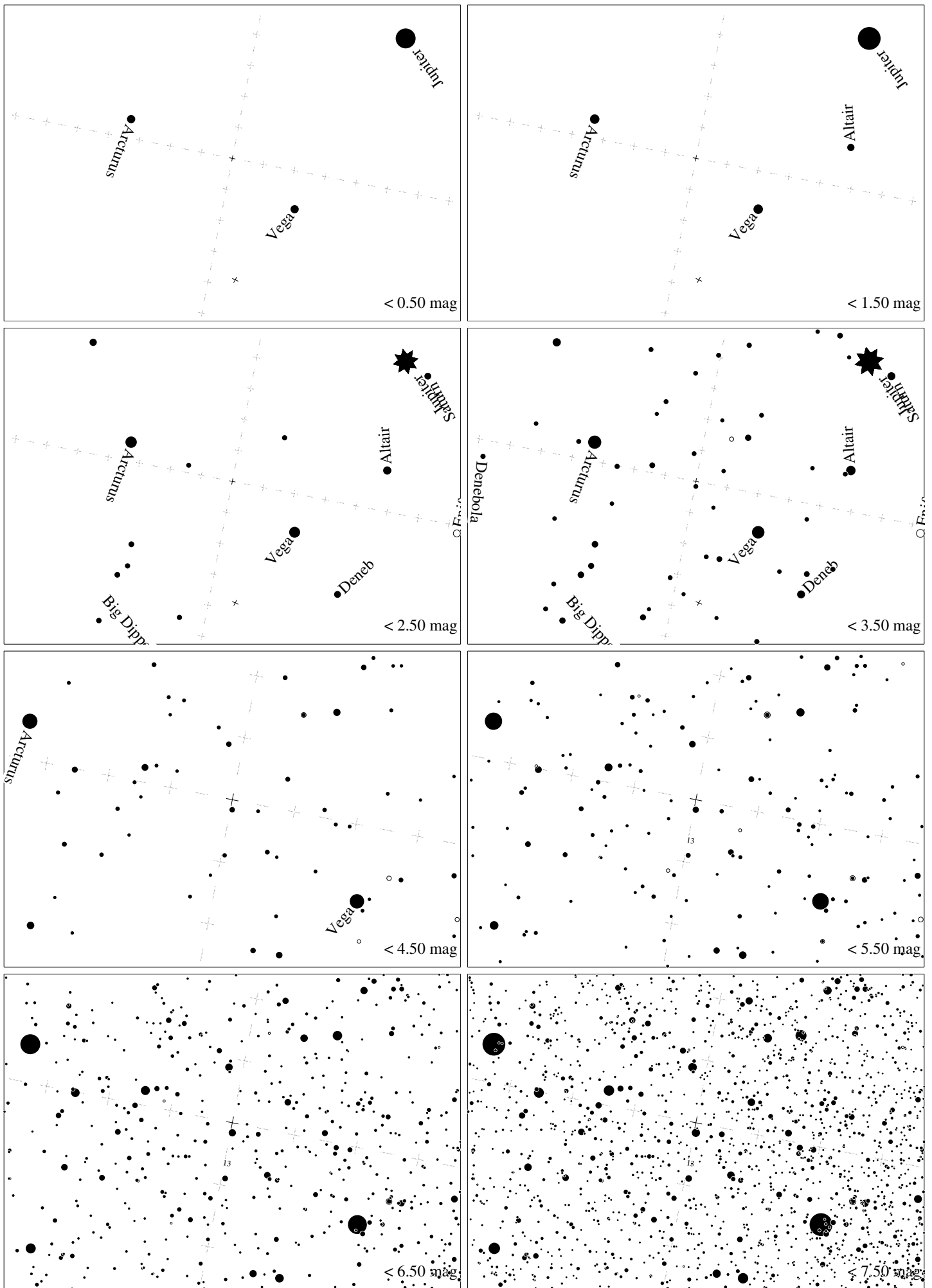
Maps for Globe at Night latitude 30^\circ , 2020-07-16, 21 h local time (Sun at -22^\circ ), transparent air. Lines from N(E,S,W) to zenith shown (crosses each 10^\circ ). Centered on \zeta Herculis, which is 11^\circ to the right from N, at 88^\circ height. Detailed maps 50^\circ vertically, the first four maps 100^\circ . Jan Hollan, CzechGlobe
