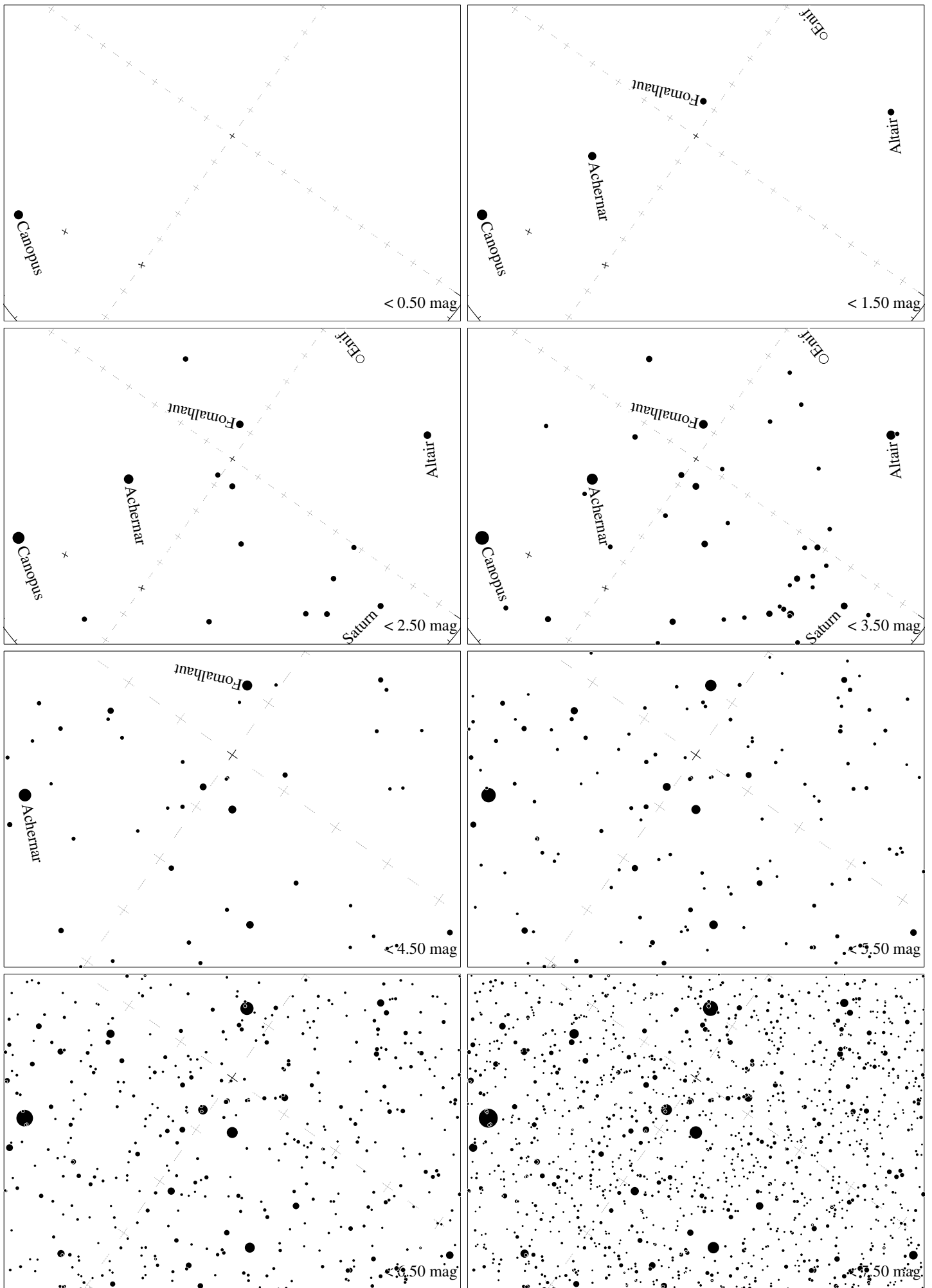
Maps for Globe at Night latitude -40^\circ , 2017-10-15, 21 h local time (Sun at -28^\circ ), transparent air. Lines from N(E,S,W) to zenith shown (crosses each 10^\circ ). Centered on Alnair ( \alpha Grus), which is 35^\circ to the right from S, at 81^\circ height. Detailed maps 50^\circ vertically, the first four maps 100^\circ . Jan Hollan, CzechGlobe
