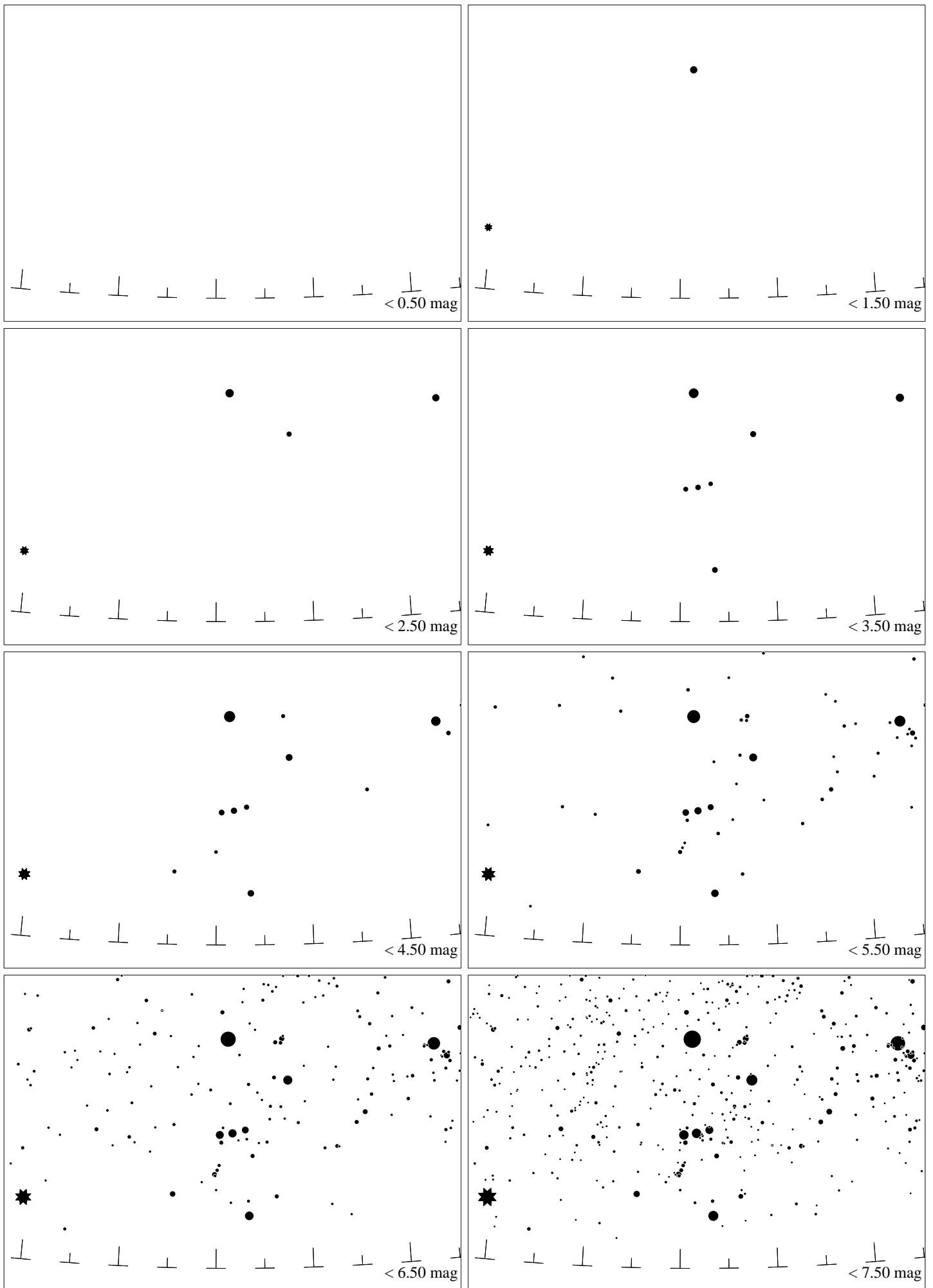
Maps for GLOBE at Night at latitude 60^\circ , March 30, 21 h local time (Mar 7, 22.5 h; Mar 23, 21.5 h; Apr 6, 20.5 h). Orion's belt is 62^\circ to the right from the south, at 14^\circ height. The brightest fixed star, Sirius, is at lower left. Jan Hollan, Ecological Institute Veronica and http://www.astro.cz/darksky
