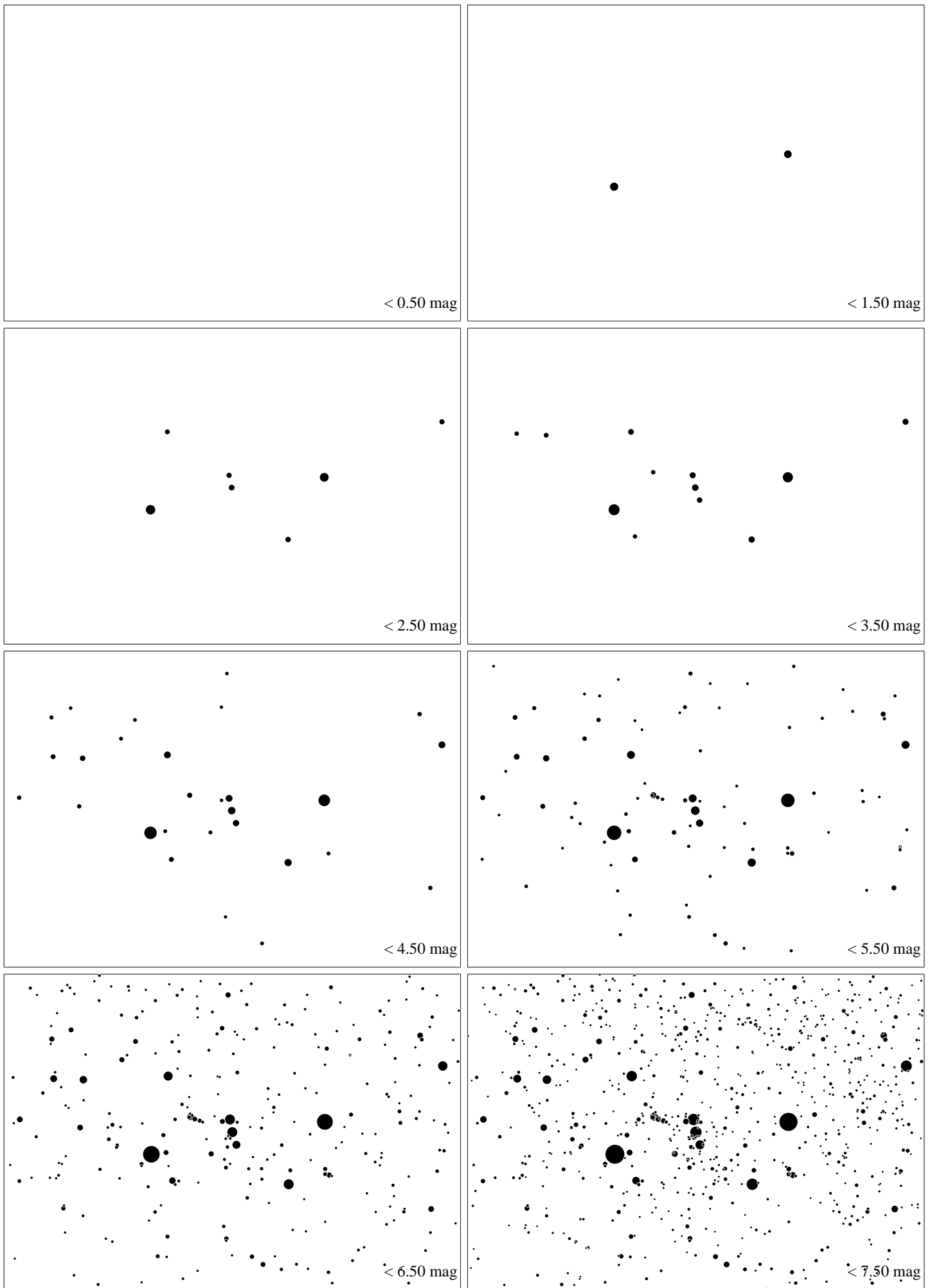
Maps for GLOBE at Night at latitude -20^\circ , March 30, 21 h local time (Mar 7, 22.5 h; Mar 23, 21.5 h, Apr 6, 20.5 h). Orion's belt is 100^\circ to the right from the south, at 30^\circ height. The brightest fixed star, Sirius, is a bit above the map. Jan Hollan, Ecological Institute Veronica and http://www.astro.cz/darksky
