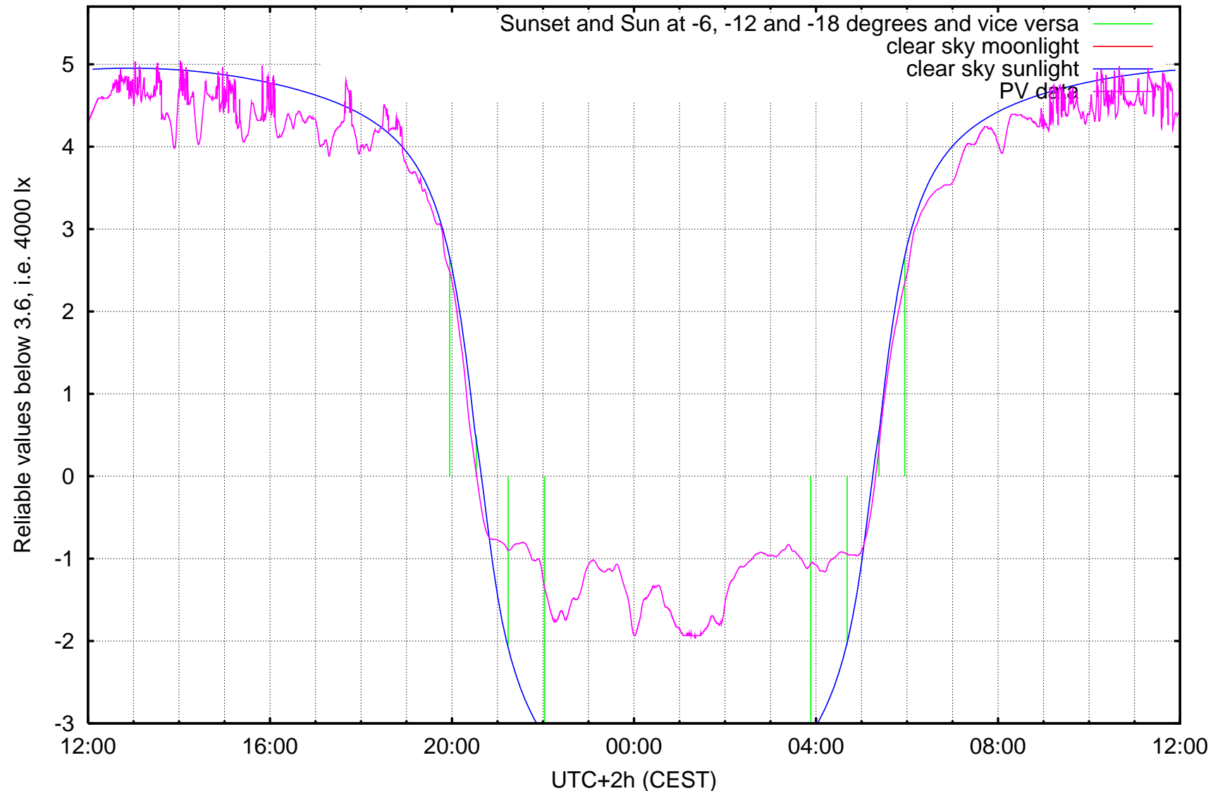
log10 ( illuminance / 1 lx ) Kravi hora, Brno, ending at Wednesday 2006-08-23 noon
