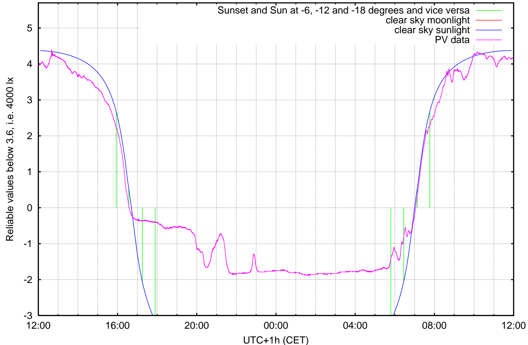
log10 ( illuminance / 1 lx ) Kravi hora, Brno, ending at Wednesday 2006-12-20 noon
