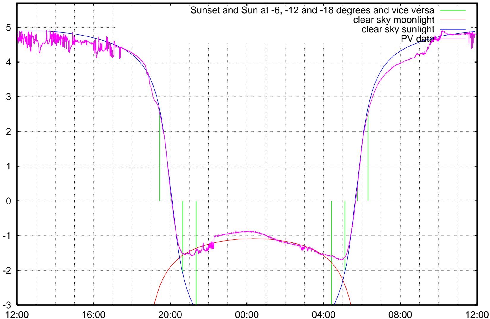
log10 ( illuminance / 1 lx ) Kravi hora, Brno, ending at Thursday 2006-09-07 noon
