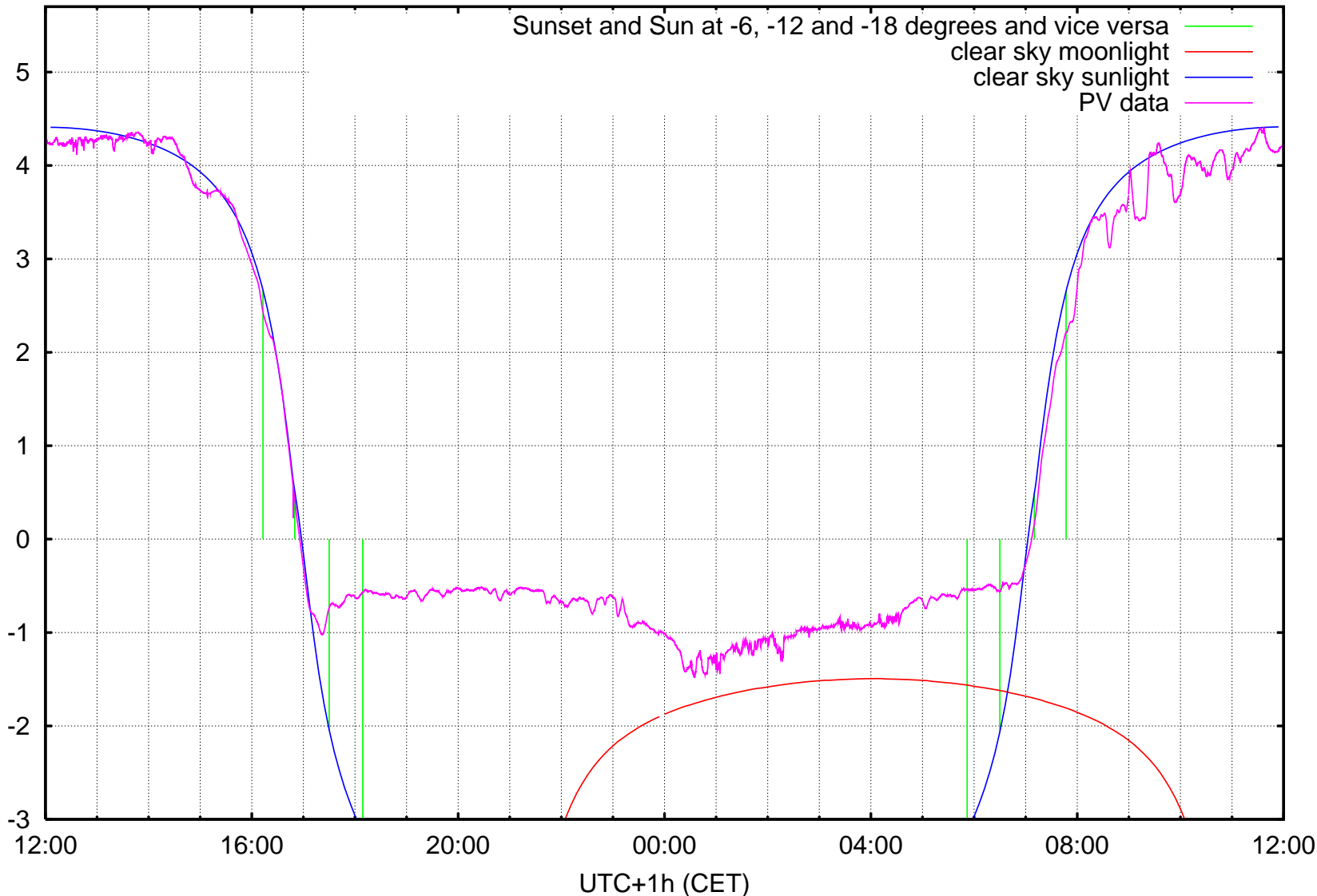
log10 ( illuminance / 1 lx ) Kravi hora, Brno, ending at Tuesday 2007-01-09 noon
