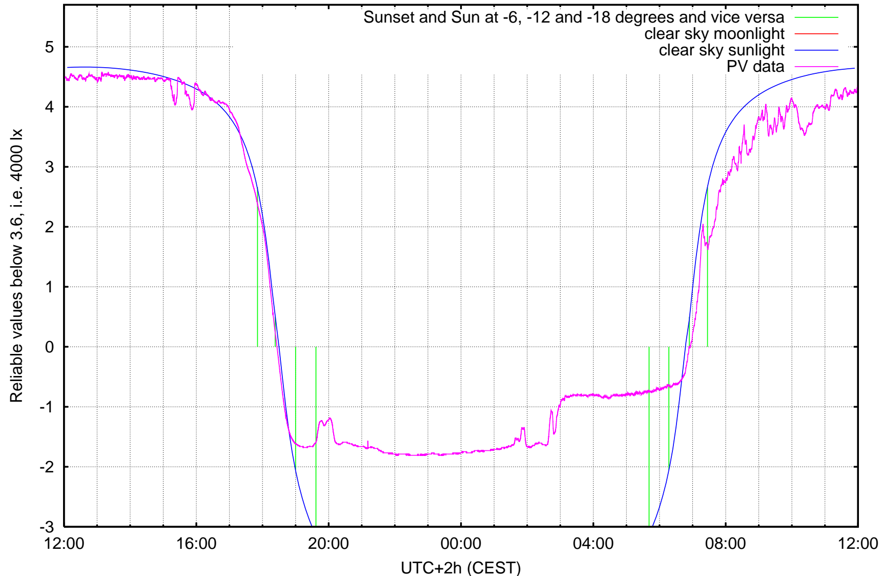
log10 ( illuminance / 1 lx ) Kravi hora, Brno, ending at Monday 2006-10-23 noon
