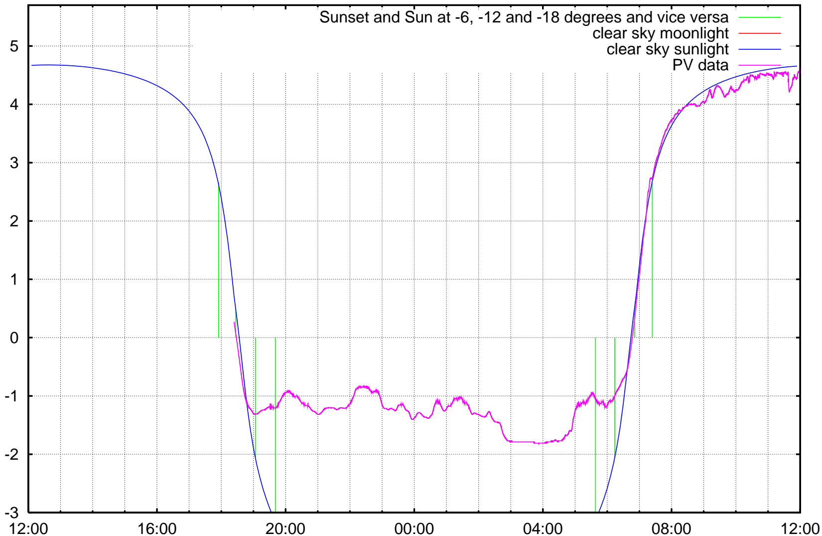
log10 ( illuminance / 1 lx ) Kravi hora, Brno, ending at Saturday 2006-10-21 noon
