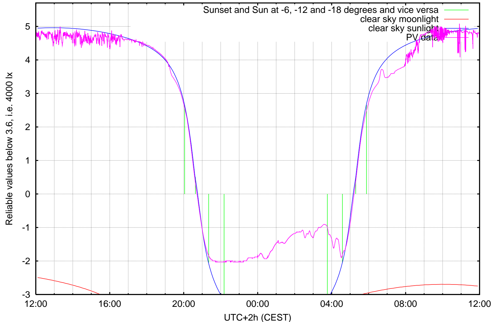
log10 ( illuminance / 1 lx ) Kravi hora, Brno, ending at Sunday 2006-08-20 noon
