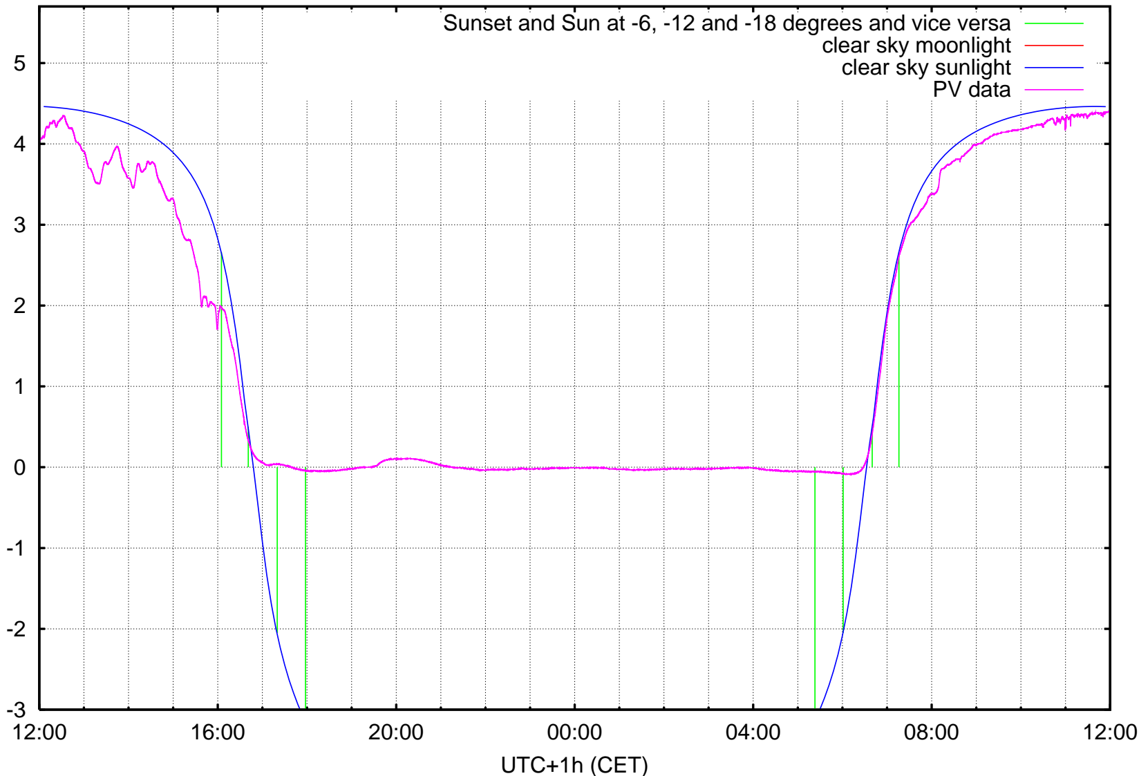
log10 ( illuminance / 1 lx ) Kravi hora, Brno, ending at Thursday 2006-11-23 noon
