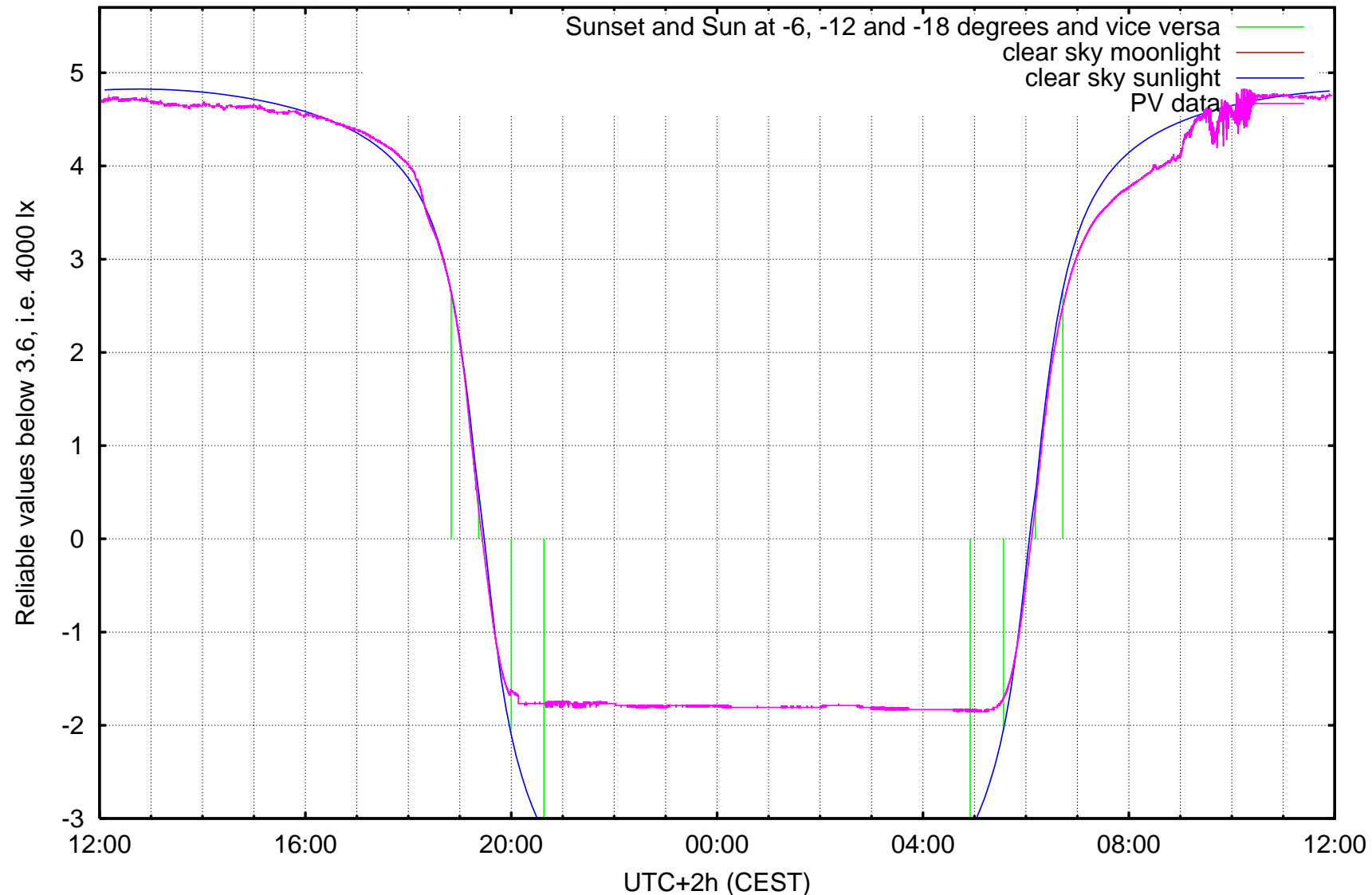
log10 ( illuminance / 1 lx ) Kravi hora, Brno, ending at Sunday 2006-09-24 noon
