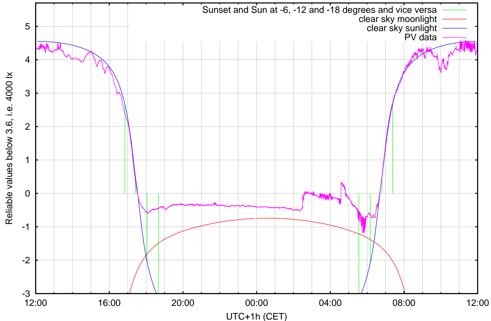
log10 ( illuminance / 1 lx ) Kravi hora, Brno, ending at Saturday 2007-02-03 noon
