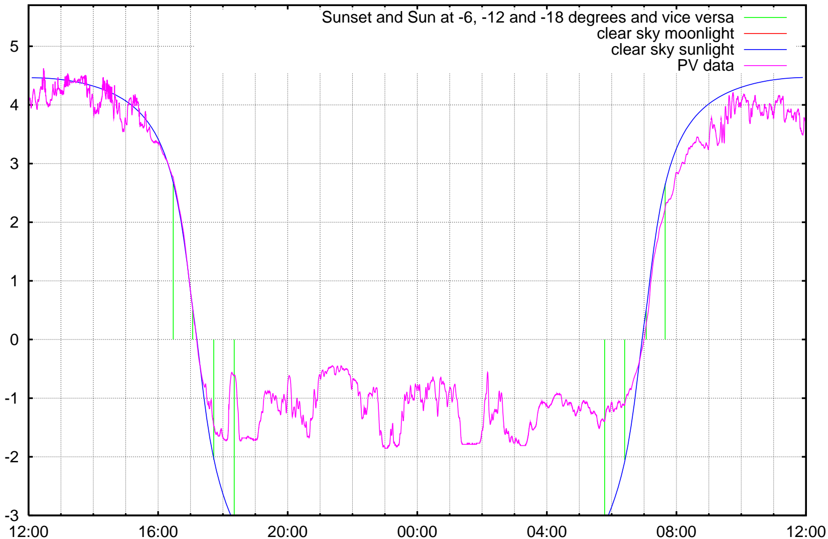
log10 ( illuminance / 1 lx ) Kravi hora, Brno, ending at Saturday 2007-01-20 noon
