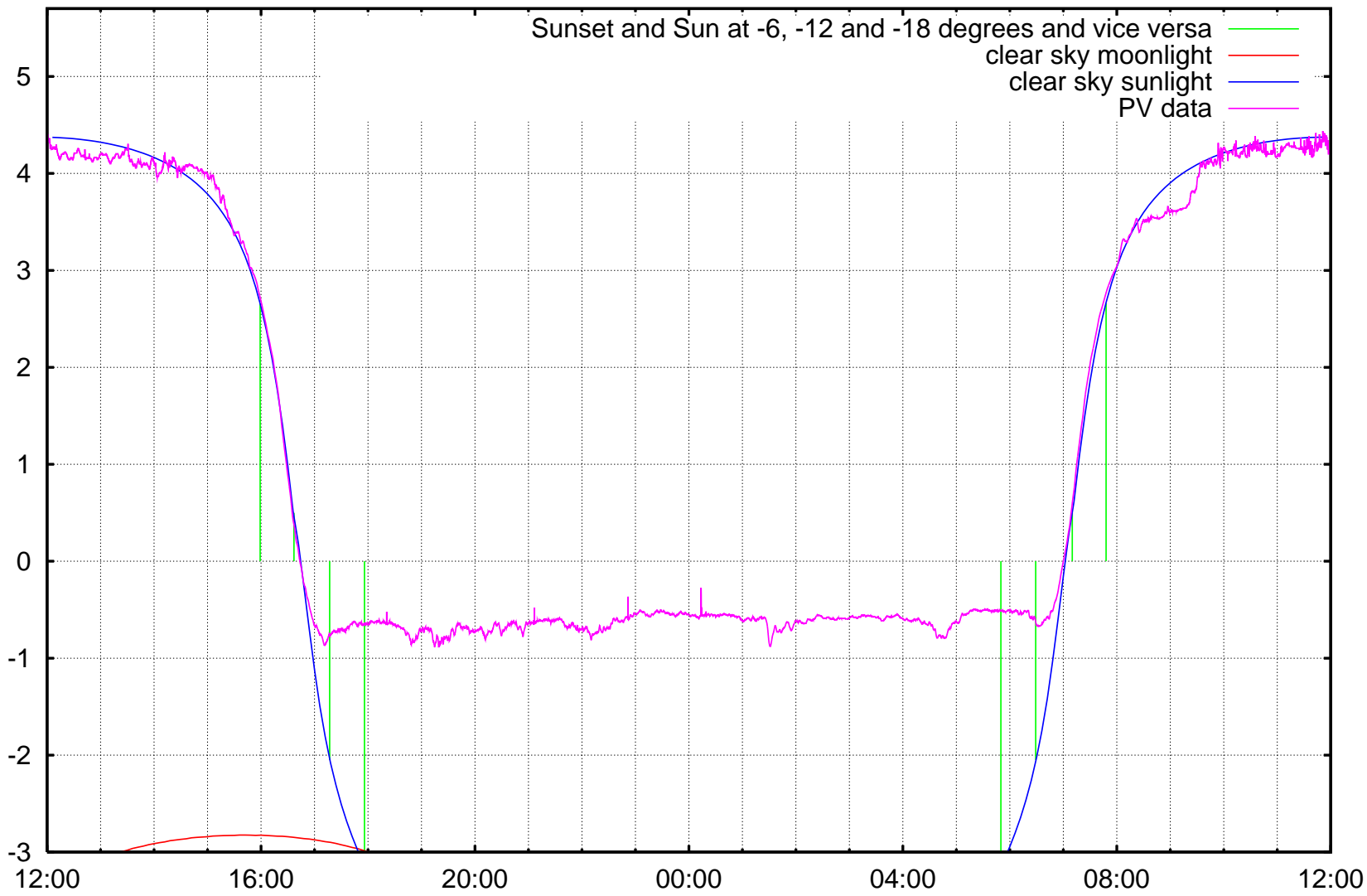
log10 ( illuminance / 1 lx ) Kravi hora, Brno, ending at Monday 2006-12-25 noon
